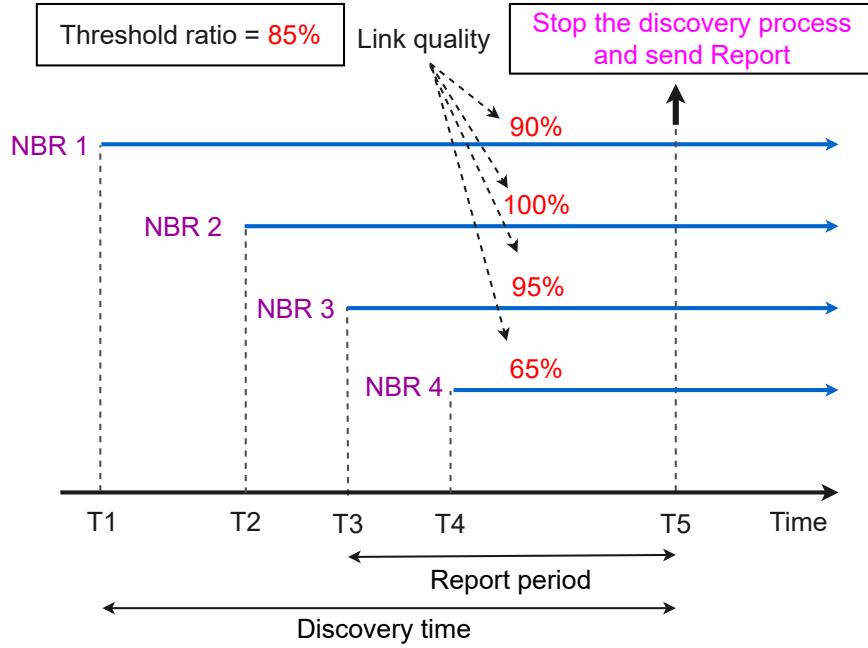
Figure 3.4: Discovery time of a joining node
