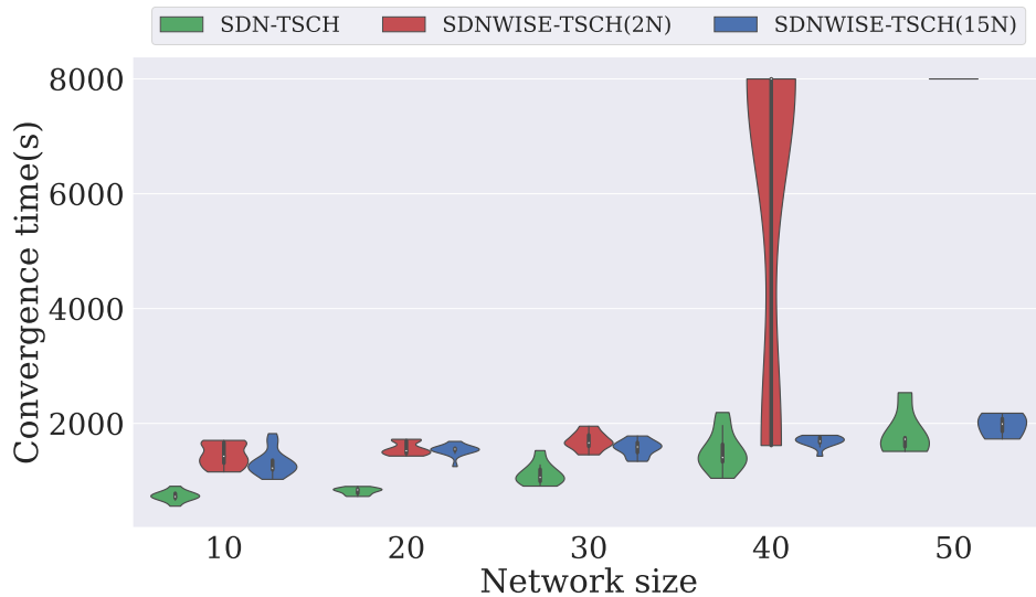
Figure 3.7: Network convergence time
