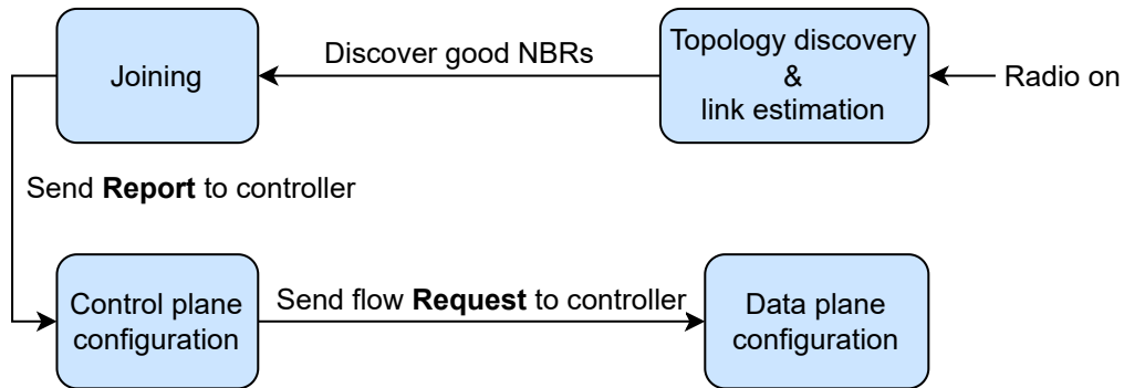
Figure 3.1: The configuration process of a new node in SDN-TSCH, (NBR = neighbor)
