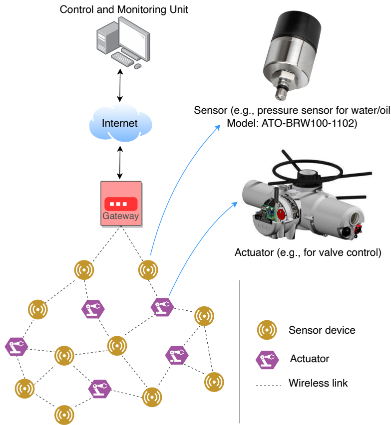
Figure 1.1: Industrial Wireless Sensor Network scenario
