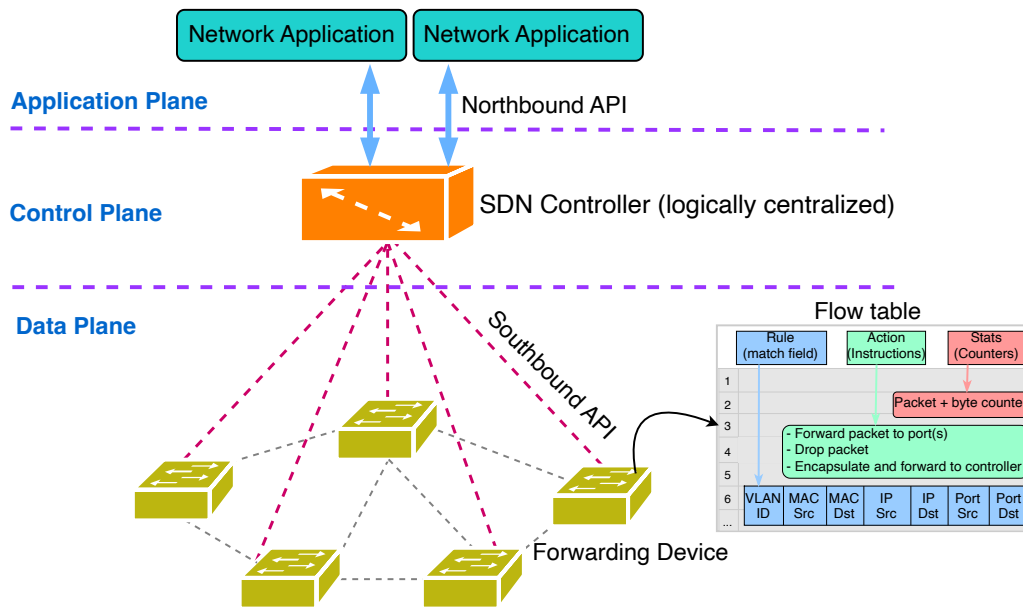
Figure 2.5: SDN architecture
