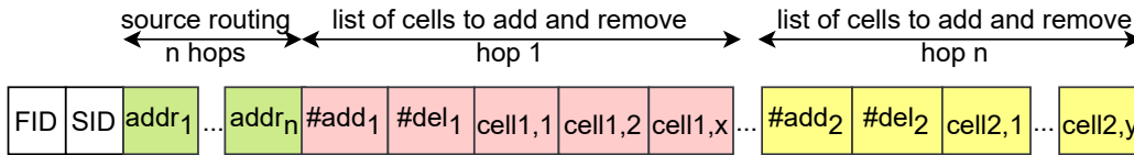
Figure 5.2: Enhanced format of config packet
