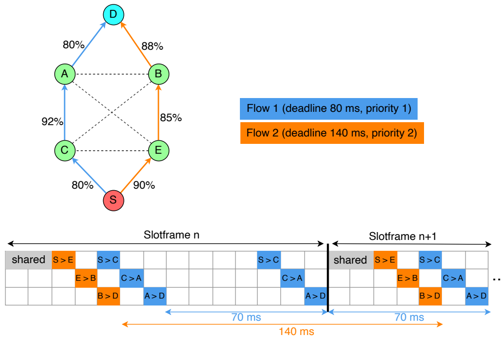
Figure 2.6: Scheduling flows with different deadlines and priority in SDNWISE-TSCH
