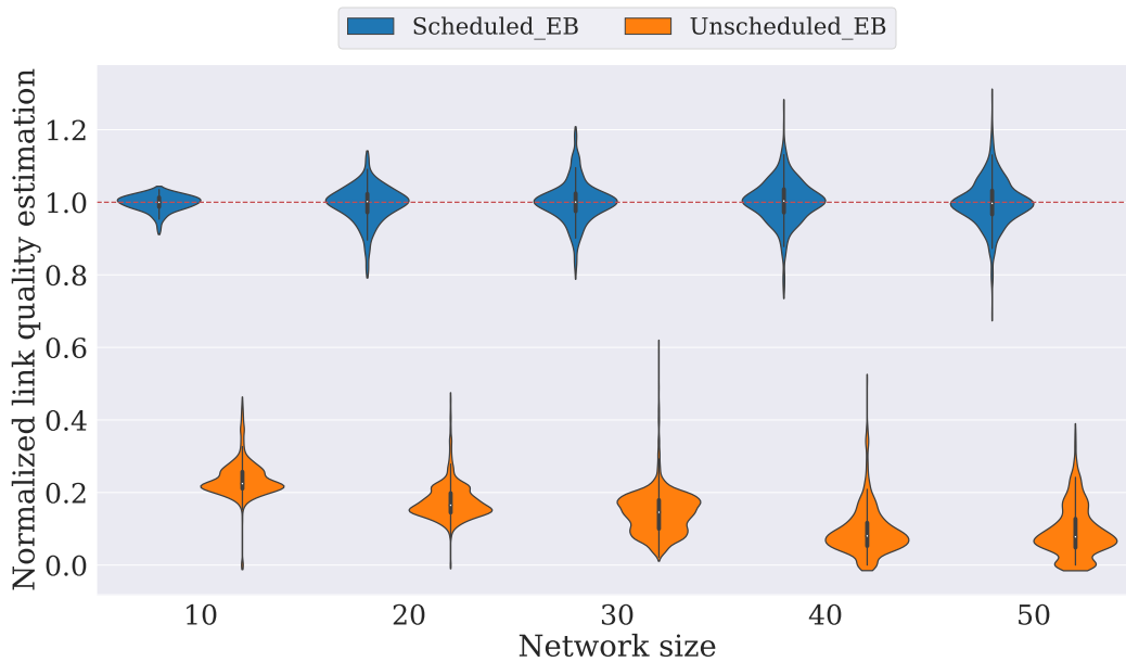
Figure 4.2: Link quality estimation
