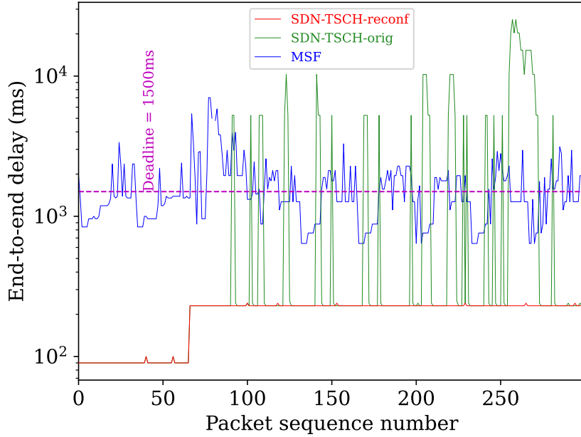
Figure 5.4: Per-packet end-to-end delay of Flow_F in each solution
