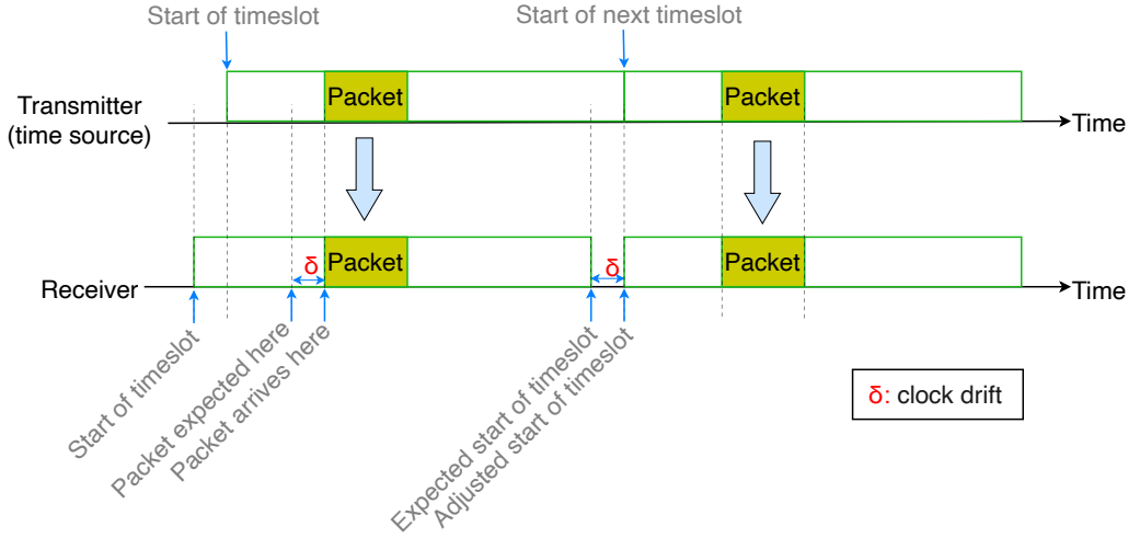
Figure 2.3: Frame-based synchronization schemes in TSCH network
