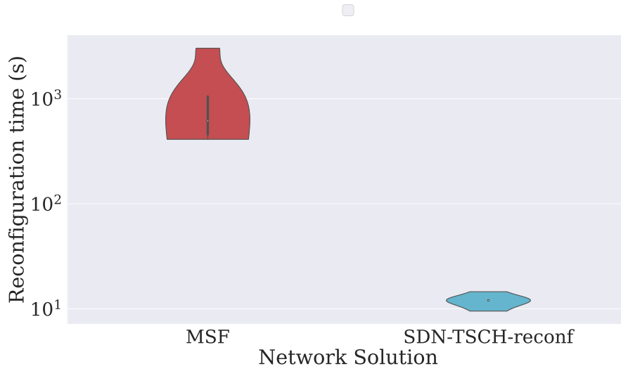
Figure 5.6: Reconfiguration time
