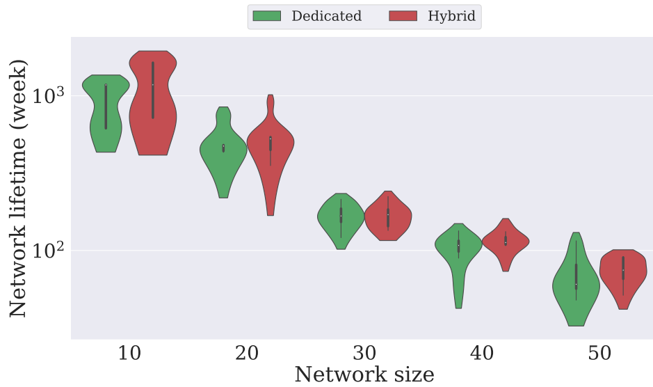
Figure 4.7: Network lifetime
