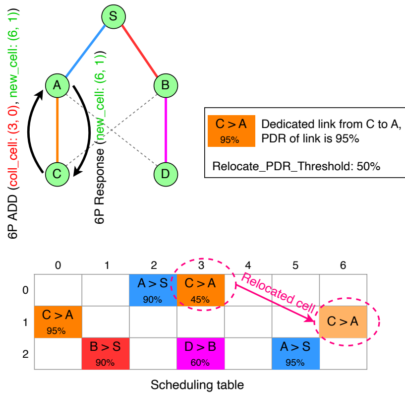
Figure 2.4: Relocation of colliding cell in MSF
