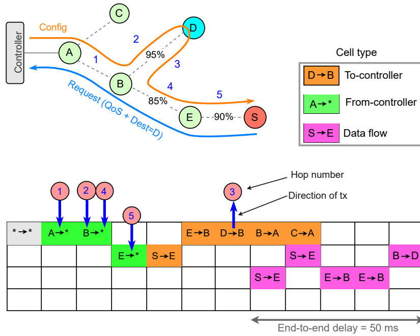
Figure 2: Data flow Configuration in SDN-TSCH
