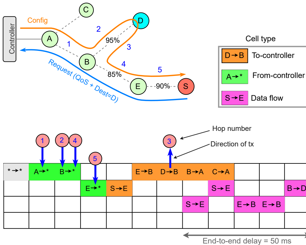
Figure 3.6: Data flow Configuration in SDN-TSCH
