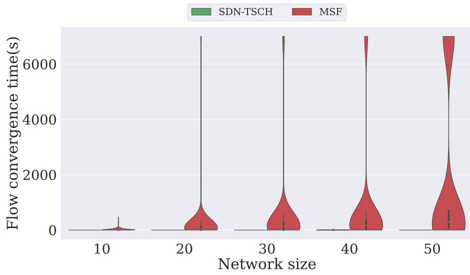
Figure 3.12: Data flow convergence time
