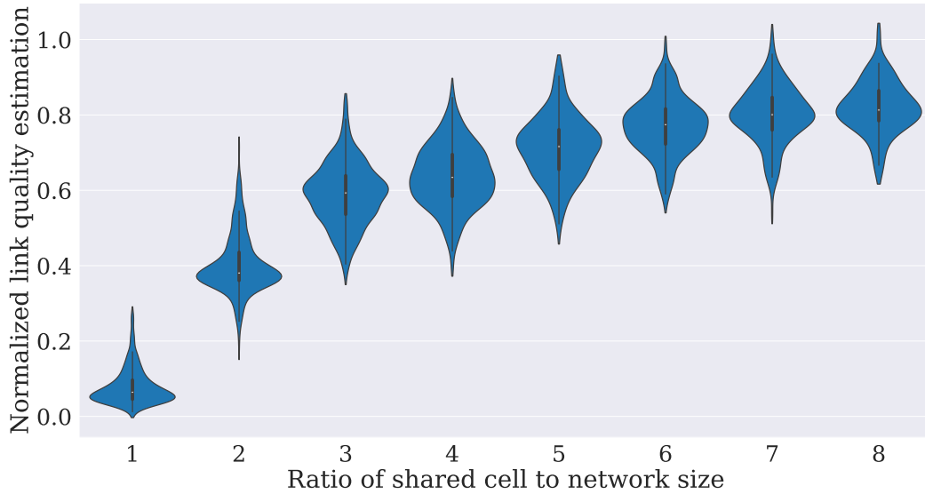
Figure 4.3: Accuracy of link quality estimation in SDN-TSCH
