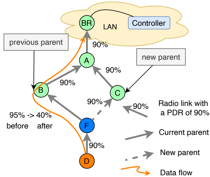
Figure 5.1: A controller needs to reconfigure the control and data planes to redirect the flows through the link (F→C) when the PDR of the link (F→B) decreases from 95% to 40%
