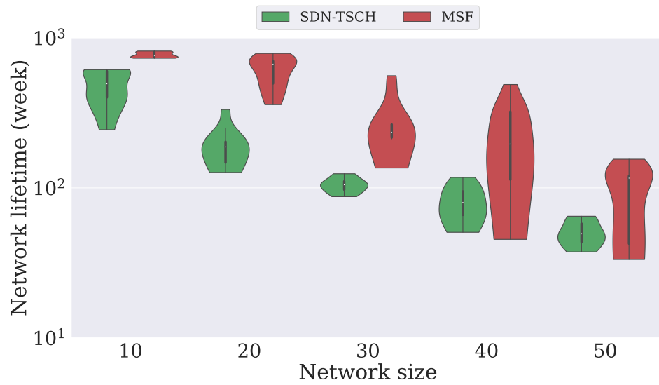
Figure 3.15: Network lifetime
