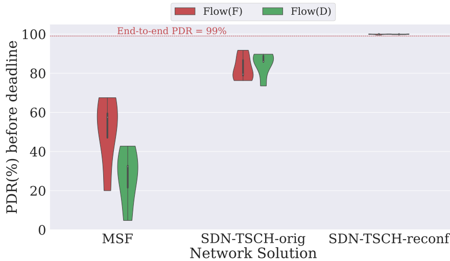
Figure 5.5: Per-flow PDR
