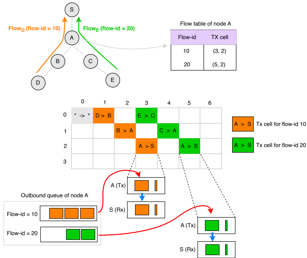
Figure 3.2: Label switching operation in SDN-TSCH
