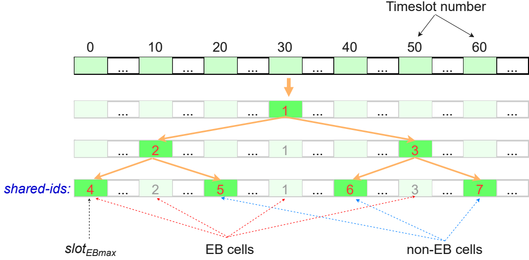
Figure 4.1: Shared cell ID allocation in slotframe for the control plane
