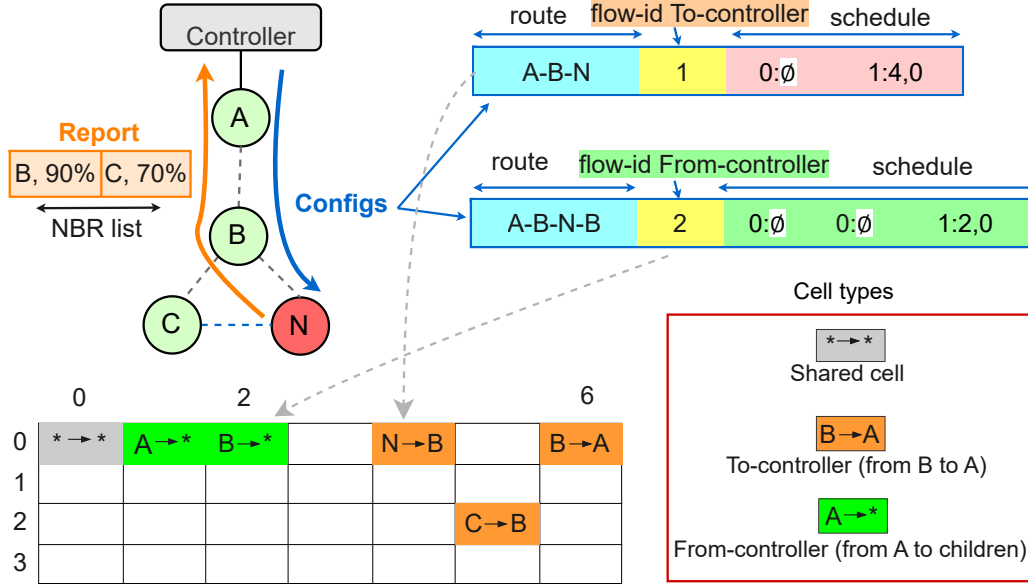
Figure 3.5: Dedicated control plane in SDN-TSCH
