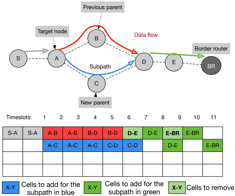
Figure 5.3: Schedule update when redirecting a data flow
