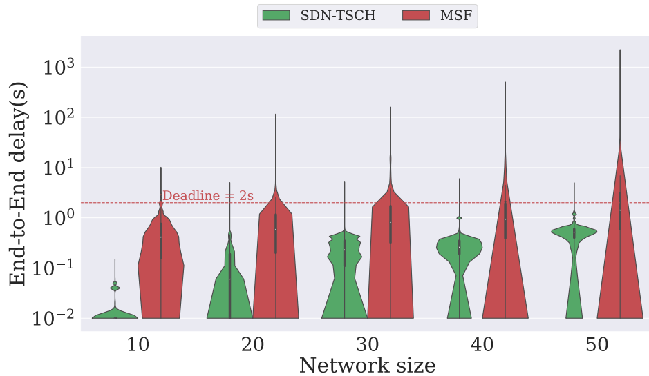
Figure 3.11: End-to-end delay
