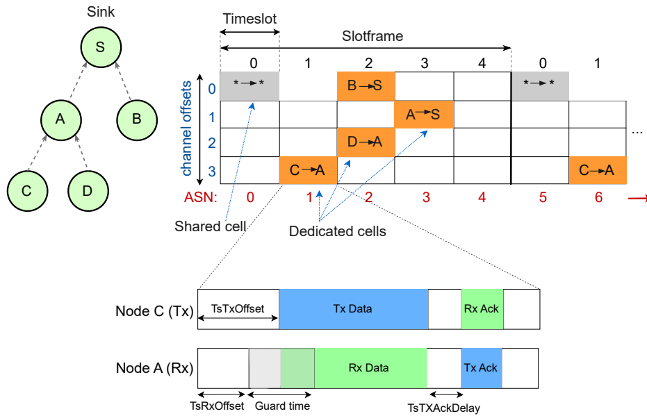
Figure 2.2: Simple TSCH schedule with shared and dedicated cells
