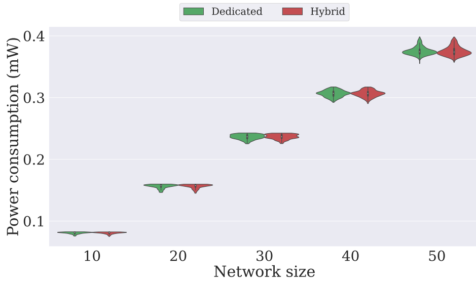
Figure 4.6: Power consumption of nodes in joining period
