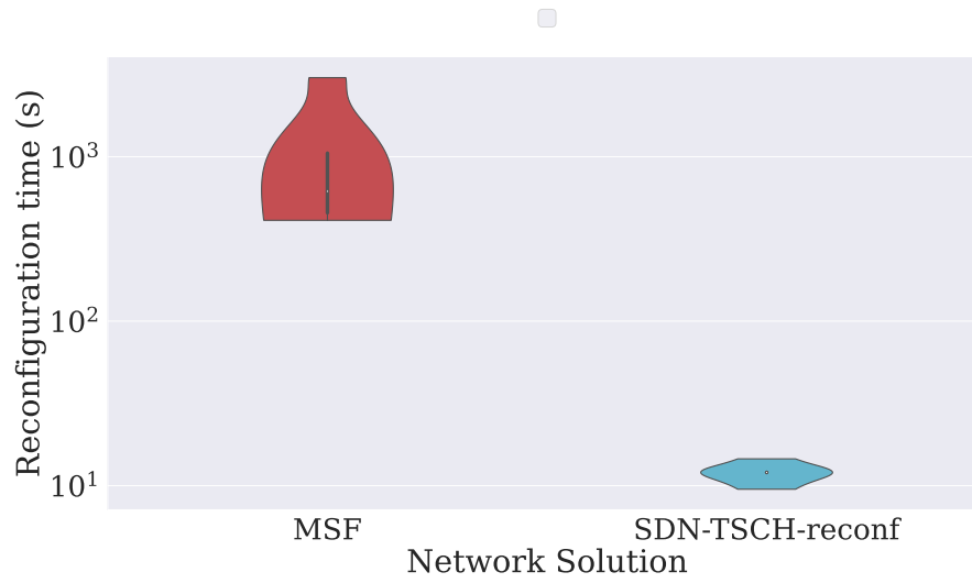
Figure 10: Temps de Reconfiguration
