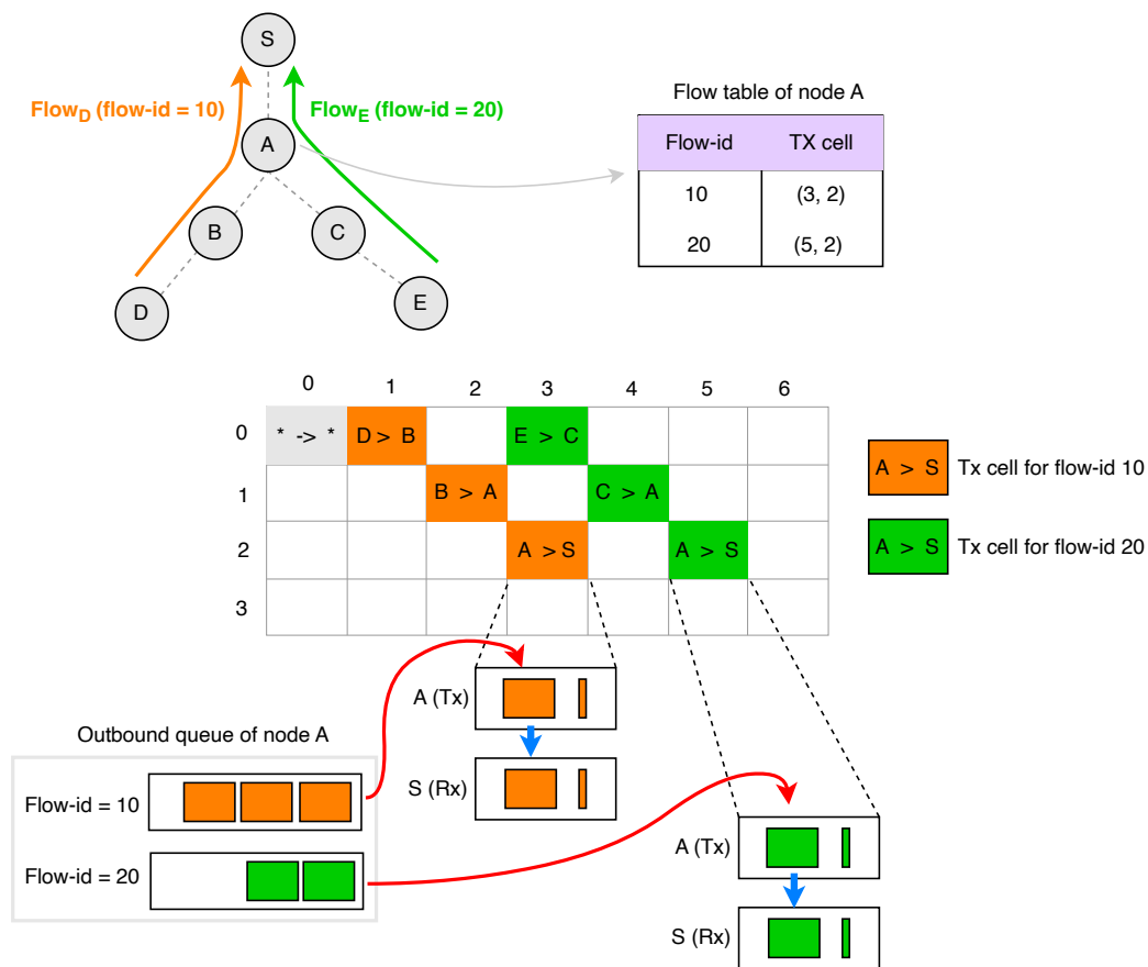
Figure 1: Label switching operation in SDN-TSCH
