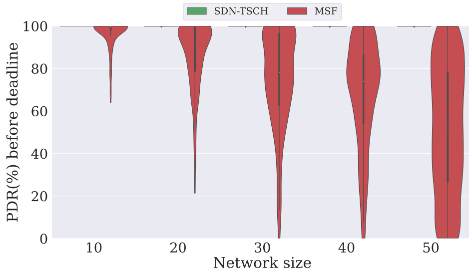
Figure 3.10: PDR of flows before deadline
