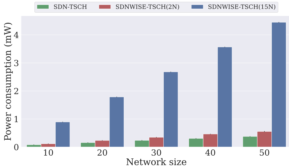
Figure 3.8: Power consumption of nodes in joining period
