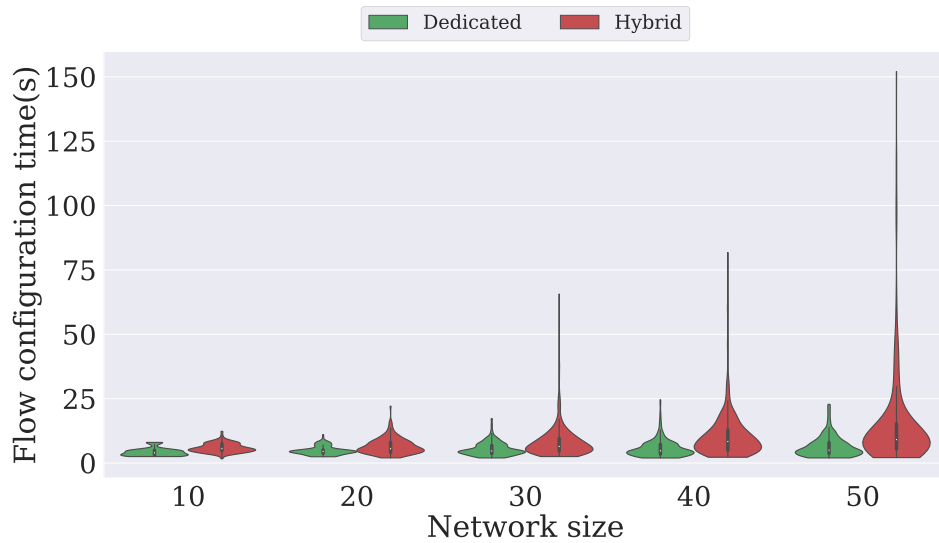
Figure 4.5: Data flow configuration time
