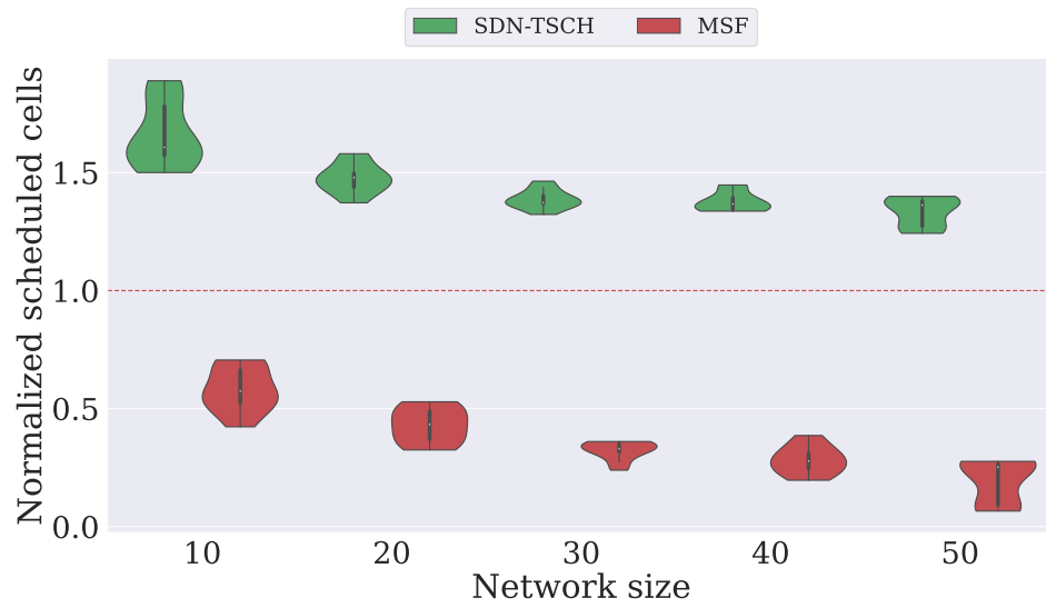
Figure 3.14: Ratio of scheduled cells
