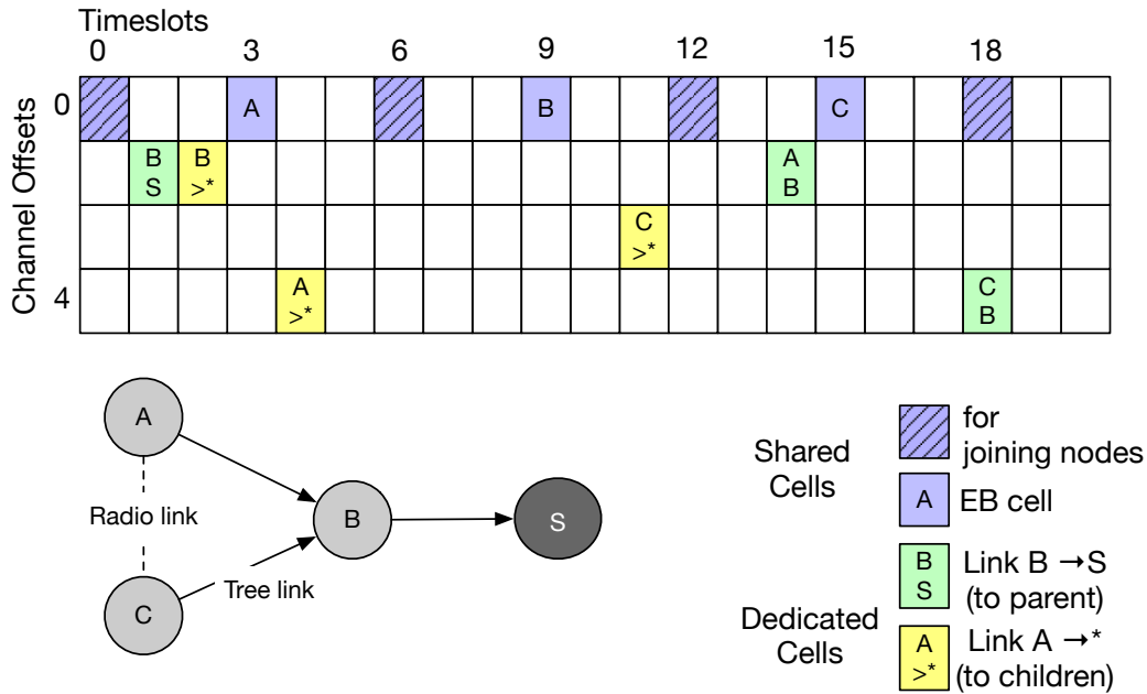
Figure 3.3: Organization of the slotframe
