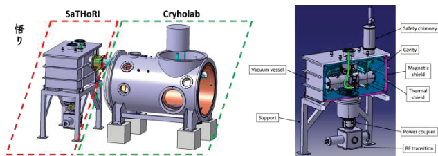
Figure 12: The SATHORI test cryostat.
