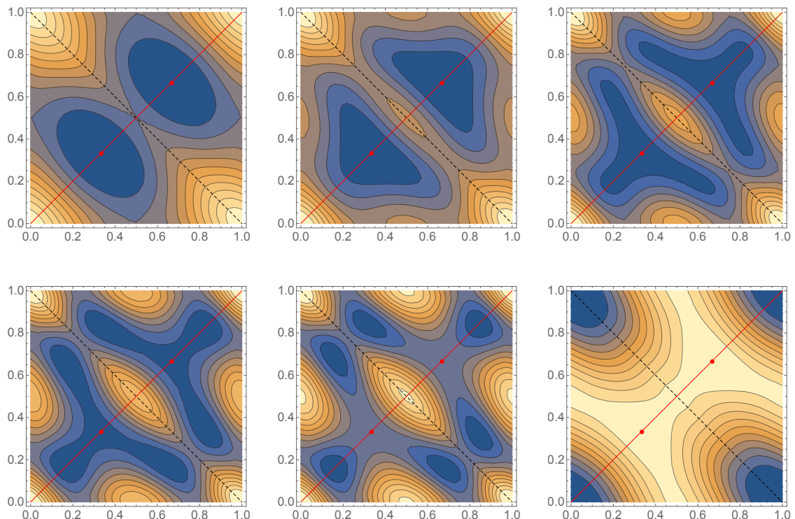
FIGURE 6.2. SU(3) background field effective potential in the fundamental parallelepiped r = x_1 \bar{\alpha}^{(1)} + x_2 \bar{\alpha}^{(2)} , with \bar{\alpha}_1 = 2\pi(1, -1/\sqrt{3}) , \bar{\alpha}_2 = 2\pi(1, 1/\sqrt{3}) and 0 < x_i < 1 . The fundamental parallelepiped is made of two Weyl chambers (separated by the dashed line) which contain each one center-symmetric or confining point, located (1/3, 1/3) and (2/3, 2/3) respectively (red dots). Finally, the charge conjugation invariant states are indicated by a red line.
