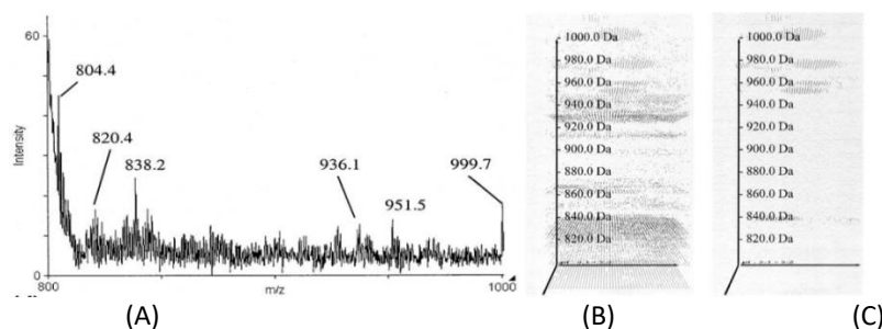
Figure 5: (A) portion of a spectrum ( m/z range of 800-1000 Da) from a collecting membrane obtained from a 2-DE separation of E. coli . (B) 3-D representation of the acquired data for the pI range from 5.1 to 5.2 on the x axis and the MW range from 45 to 35 kDa on y axis. Background noise signal is clearly and homogeneously distributed all over the surface such as 804.4 Th peak visible in (A). (C) Remaining signal after background noise suppression highlighting well localized signal such as peak 999.7 Da. (Adapted from [44])
