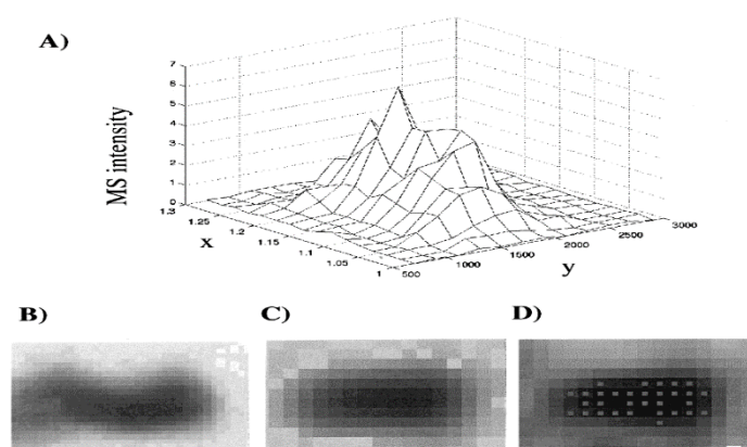
Figure 4: Two-dimensional MS scan of the 1-DE of soybean trypsin inhibitor (ITRA) band blotted on a PVDF membrane ( 1.1 \times 0.9 \text{ cm}^2 ) and sprayed with a 10 mg/mL ACCA solution in 70% methanol. An array of 16 \times 12 points was defined around the centre of the band. (A) 3-D MS intensity profile. All m/z higher than 1100 Th were considered to create the smoothed image. (B) Amido black-stained image. (C) MS intensity image. (D) MS intensity image, plotted in a logarithmic scale. The white dots represent the positions where the ITRA was unambiguously identified with a minimum of 5 m/z matching values with PeptIdent. (Adapted from [38])
