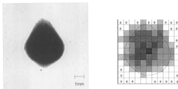
Figure 2: Optical image of the transthyretin (TTR) protein blotted on PVDF membrane after 2-DE separation and image generated from the data acquired by IR-MALDI scanning. For the mass spectrometry experiment, the investigated blot area (TTR spot) was divided into an array of 121 ( 11 \times 11 ) 500 \times 500 \mu\text{m}^2 squares and the signal intensity averaged over 10 spectra for each square. The contour line of the UV laser densitograph was transferred into the 2D grey-scale histogram for ease of comparison (adapted from [31]).
