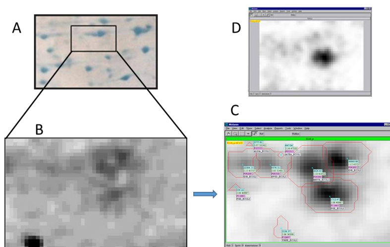
Figure 6: (A) 2-DE separation of an E. coli sample blotted on a PVDF membrane and amido black stained. The 2-DE gel was prepared in duplicated and treated by DPD. A 9 x 13 mm area was cut from the collecting membrane (pI from 5.1 to 5.2, MW from 35 to 45 kDa) and scanned every 300 mm by MALDI-MS. (B) The 1536 spectra obtained were automatically treated for peak detection, calibration and used to recreate the MS intensity image. (C) The image is enriched with PFM protein identification results and proteins spot are defined. (D) Image generated with the intensity of MALDI-MS signal within 2025 \pm 0.7 Th. The region where these masses are detected corresponds to the PGK_ECOLI spot.
