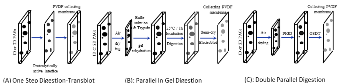
Figure 3: Schematic summary of the 3 proposed parallel digestions: (A) OSDT, (B) PIDG and (C) DPD.
