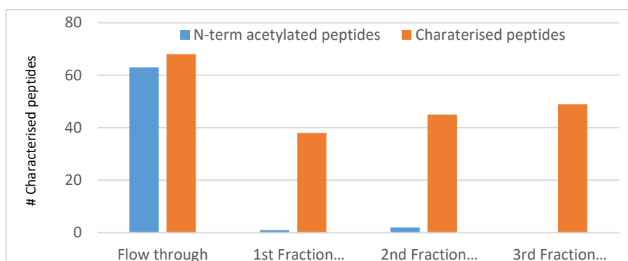
Figure 8: Distribution of the NTAed peptides characterised in human CD8 T lymphocytes after SCX separation of 100 µg of Lys-N digested sample using 20, 90, 500 mM of NaCl for peptides elution.
