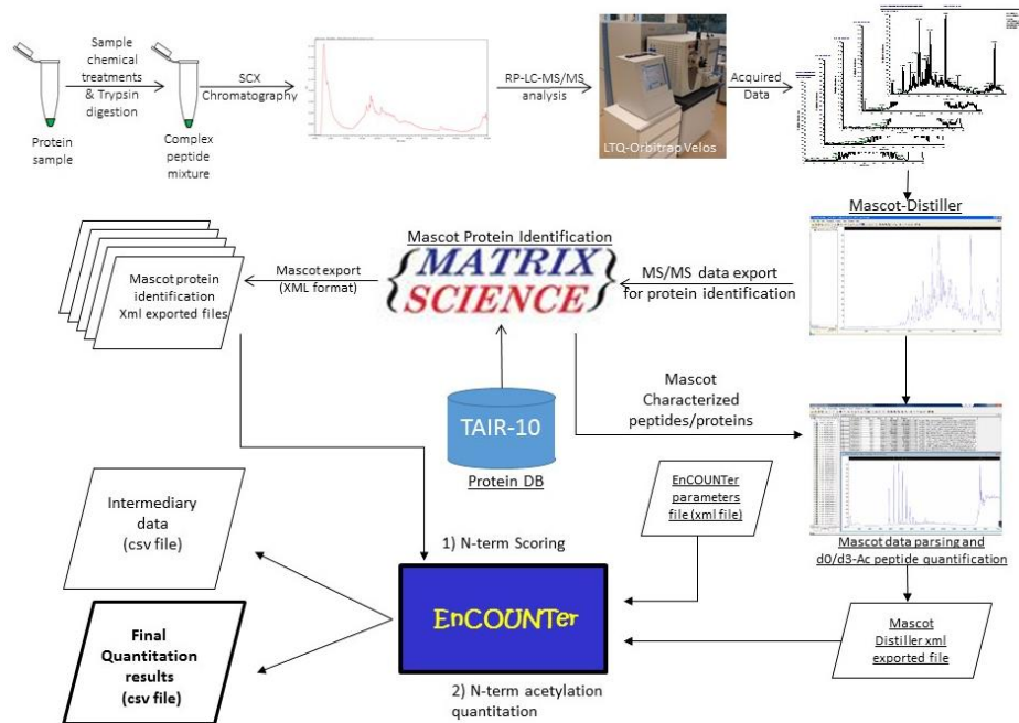
Figure 9: Overview of the SILProNAQ processing scheme: from sample to identification of mature N-terminus position and determination of NTA yield. Adapted from [99]
