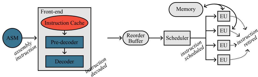
Figure 2.4: Schematic view of a CPU and life cycle of an instruction
