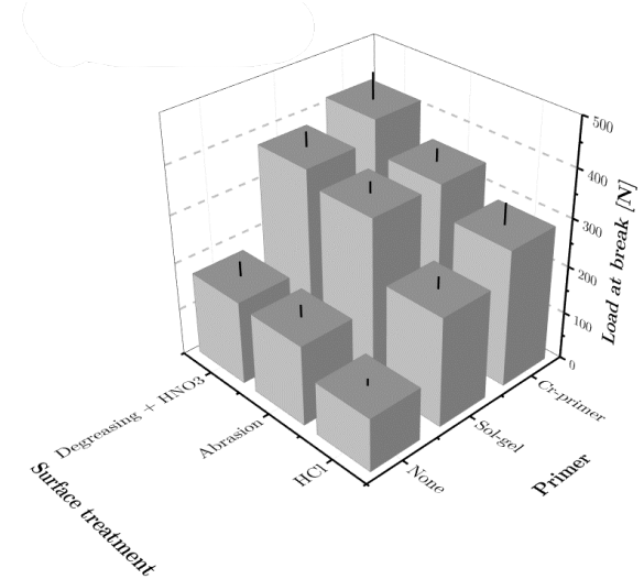
Figure 2.15: Adherence measured during the three-point bending test : Al 2024 substrate, Hysol EA 9334 adhesive, and a combination of 3 primers and 3 surface treatments. All failures are interfacial (adhesive).
