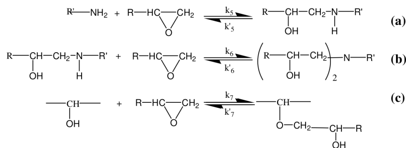
Figure 2.22: Reaction mechanisms of epoxide-amine reactions.
