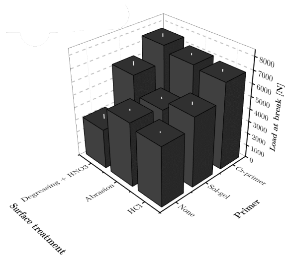
Figure 2.14: Adherence measured during the single-lap joint test : Al 2024 substrate, Hysol EA 9334 adhesive, and a combination of 3 primers and 3 surface treatments. All failures are cohesive (in the adhesive).
