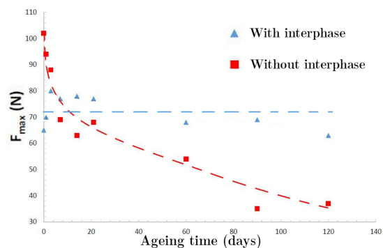
Figure 2.38: Variation in adherence of a DGEBA-DETA coating on an Al 1050 alloy substrate as a function of hygrothermal ageing time (6°C, 85% relative humidity), adapted from Pomes-Hadda [2015].
