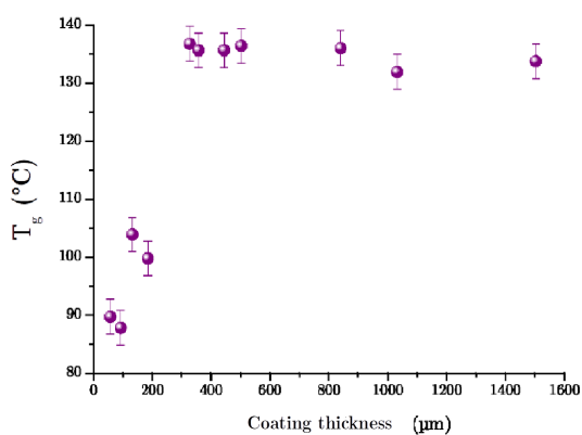
Figure 2.34: Variation in the glass transition temperature as a function of the thickness of DGEBA-DETA coatings on an Al 1050 alloy substrate, adapted from Aufroy [2005].
