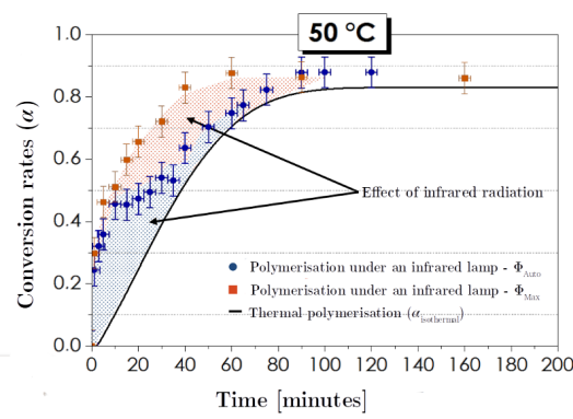
Figure 2.26: Conversion rate as a function of time for the DGEBA-TETA mixture, polymerised at 50°C in an oven and under an infrared lamp by modulating the luminous flux (automatic \approx 1500 \text{ W.m}^2 or maximum \approx 5000 \text{ W.m}^2 ), adapted from Genty [2018].
