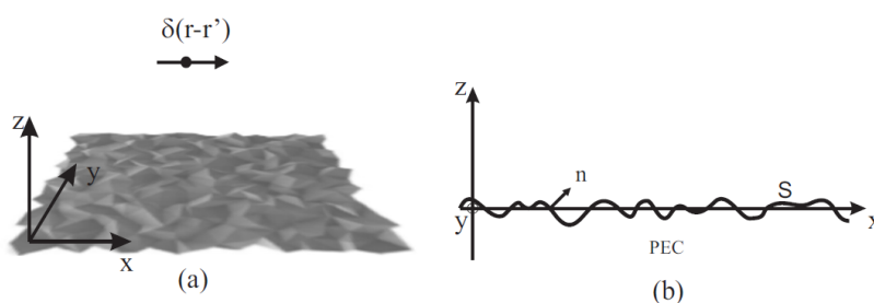
Figure 3.6 Geometry for the Green’s function problem.
