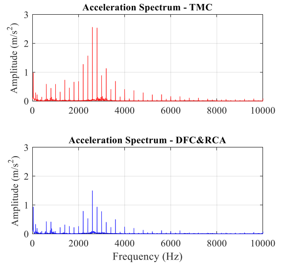
Fig. 20 Experimental results of vibration acceleration at 2000 r/min and 0.6 N·m.
