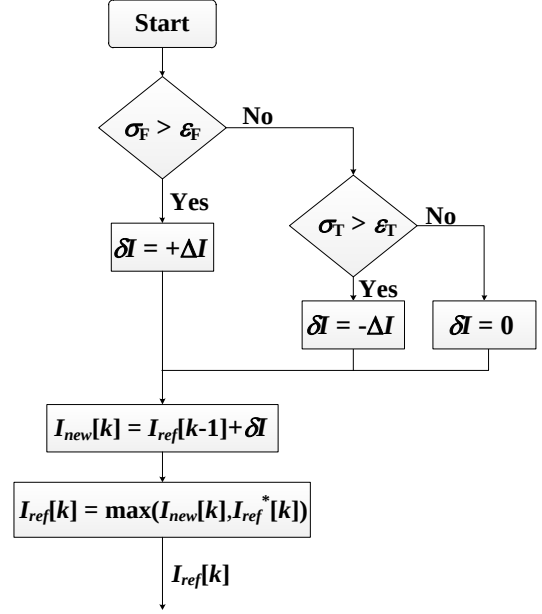
Fig. 12 Current adapter algorithm.
