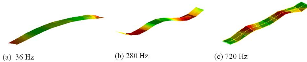
Figure IV.15. Vibration modes of the CFB.
