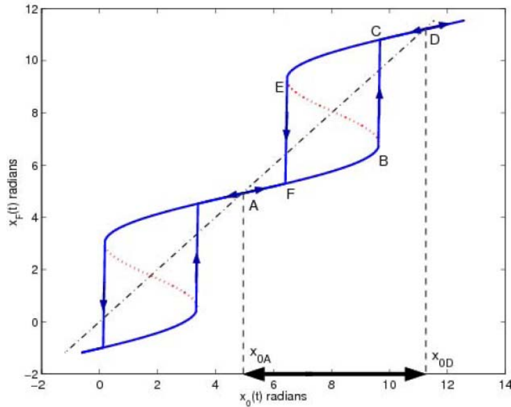
Figure II.10. The F function showing hysteresis ( C=3 and a=5 ): the numerical resolution of equation (2.5) in dotted pink line compared to the physical behavior of the laser diode in blue bold line.
