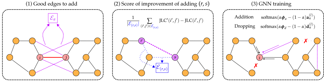
Figure 4.3: The pipeline of the proposed SJLR algorithm. SJLR first saves potential good edges \mathcal{E}_a to add to the graph based on the JLC metric. Secondly, SJLR computes the improvement score of adding these new edges as the average of the JLC improvement that concerns these edges. Thirdly, edges are added and removed according to some probability distribution during the graph neural network training.
