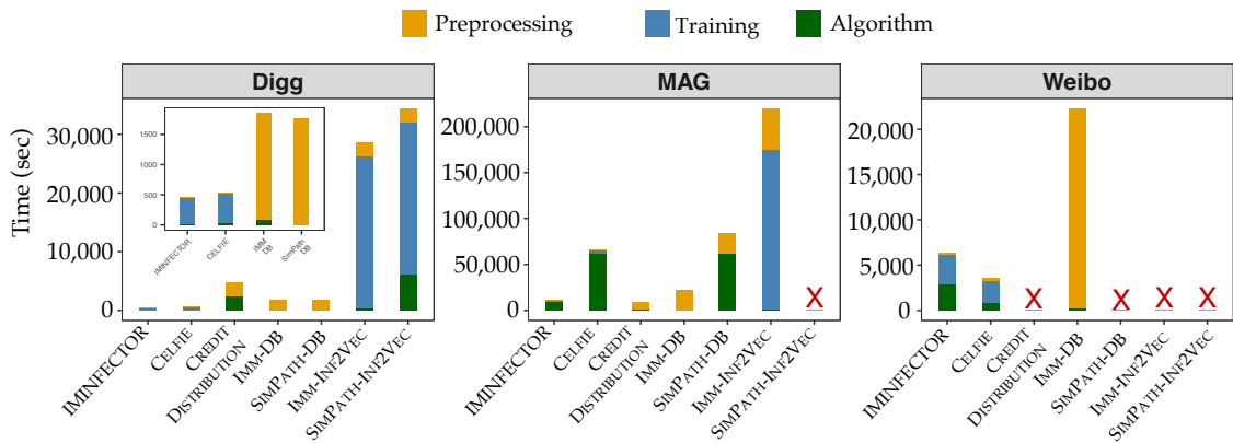
Figure 5.3: Time comparison of different models. Methods that could not scale to the dataset size are marked with \times .
