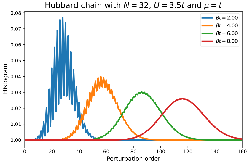
Figure 2: Histograms of the absolute contributions from different perturbation orders to the partition function of the one-dimensional Hubbard chain with N = 32 sites, U = 3.5t and \mu = t . The histograms correspond to four different temperatures and it is seen that the average perturbation order increases linearly with inverse temperature \beta .
