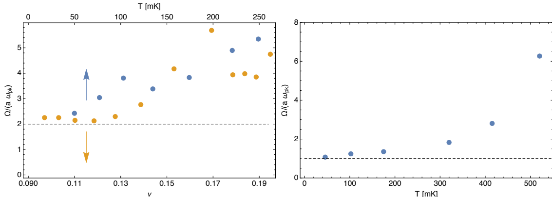
Figure 7. Ratio of coefficients suggests different dissipative mechanisms are at work in the less disordered and more disordered samples. Left: The low temperature/low filling behavior of the cleaner samples (leftmost and center plots in Fig. 6) is consistent with dissipation into mobile dislocations, shown as a dashed black line. Right: The low temperature behavior of the more disordered sample (rightmost plot in Fig. 6) is consistent with the universal phase dissipation into currents, shown as a dashed black line.
