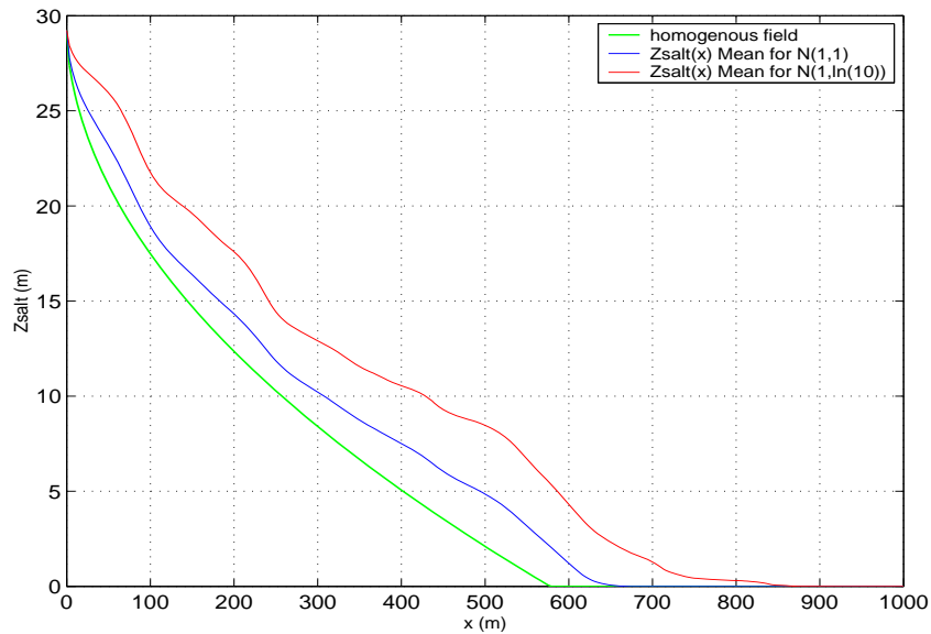
Fig. 4 Mean Z_{SALT}(x) profile transverse to seashore for a 300 \times 300 grid : analytical solution for \sigma = 0 and computed mean profiles for \sigma = 1.0 to \ln 10 ( Z_{SALT} increases with \sigma )
