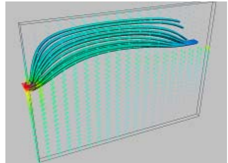
Unsaturated aquifer modelling: Vector plot of fluxes and streamlines
