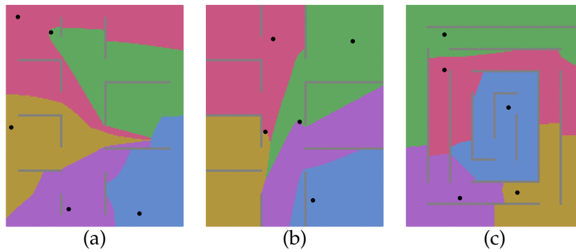
FIGURE 7.7: Scenario 5 - The results computed by the Voronoi-base method when the non-uniform density function is applied. (a): Open rooms; (b): Rooms; (c): Spiral.
