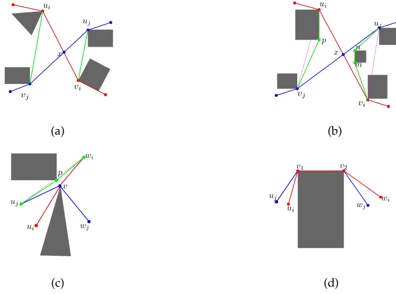
FIGURE 4.4: Top (Case 1): \pi_i (in red) and \pi_j (in blue) contain two crossing segments \overline{u_i v_i} and \overline{u_j v_j} . (a): \overline{u_i v_i} and \overline{u_j v_i} (in green) do not cross obstacles and |u_i v_j| + |u_j v_i| < |u_i v_i| + |u_j v_j| . (b): \overline{u_i v_i} and \overline{u_j v_i} (dotted lines) cross obstacles but \pi_{ij} = \langle u_i, p, v_j \rangle and \pi_{ji} = \langle u_j, n, m, v_i \rangle (in green) do not cross obstacles and |\pi_{ij}| + |\pi_{ji}| < |u_i v_i| + |u_j v_j| . Bottom (Case 2): \pi_i (in red) and \pi_j (in blue) cross at a common vertex. (c): By swapping w_i and w_j we obtain non crossing paths which are not shortest paths ( |\langle u_j, p, w_i \rangle| < |\langle u_j, v, w_i \rangle| ). (d): By swapping w_i and w_j we obtain non crossing paths that have the same length.
