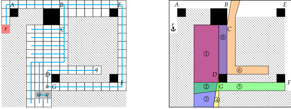
FIGURE 6.8: An example showing that the search of a maximum tree in \hat{G}_{cfg} is a suboptimal solution. Left: the cyan path is an optimal solution found in G_{cfg} that can cover all the cells in the workspace. Right: a partition (incomplete) of the workspace associated with G_q . The small regions between I_2, I_5 and the obstacle with apex D can be ignored compared to the discretization precision.
