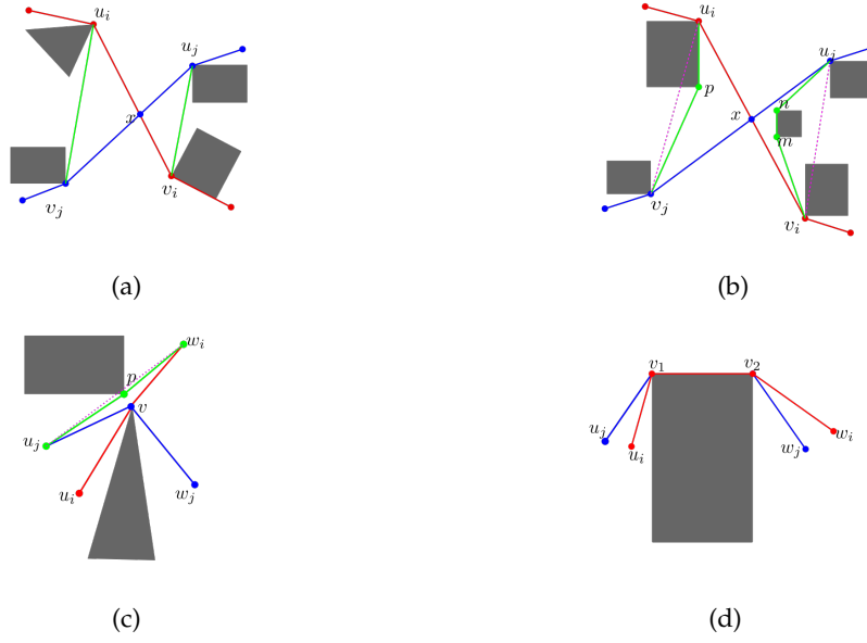
FIGURE 4.4: Top (Case 1): \pi_i (in red) and \pi_j (in blue) contain two crossing segments \bar{u}_i\bar{v}_i and \bar{u}_j\bar{v}_j . (a): \bar{u}_i\bar{v}_j and \bar{u}_j\bar{v}_i (in green) do not cross obstacles and |u_i v_j| + |u_j v_i| < [u_i v_i] + |u_j v_j| . (b): \bar{u}_i\bar{v}_j and \bar{u}_j\bar{v}_i (dotted lines) cross obstacles but \pi_{ij} = \langle u_i, p, v_j \rangle and \pi_{ji} = \langle u_j, n, m, v_i \rangle (in green) do not cross obstacles and |\pi_{ij}| + |\pi_{ji}| < |u_i v_i| + |u_j v_j| . Bottom (Case 2): \pi_i (in red) and \pi_j (in blue) cross at a common vertex. (c): By swapping w_i and w_j we obtain non crossing paths which are not shortest paths ( |\langle u_j, p, w_i \rangle| < |u_j, v, w_i| ). (d): By swapping w_i and w_j we obtain non crossing paths that have the same length.
