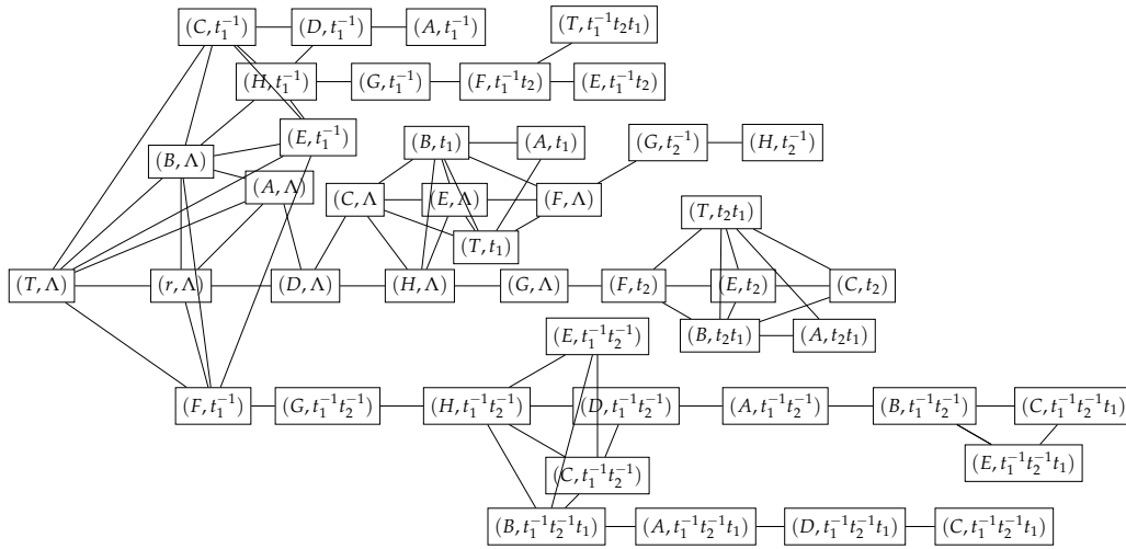
FIGURE 2.7: An example of the homotopy augmented visibility graph G_{hvis} associated with the workspace in Fig. 2.1.
