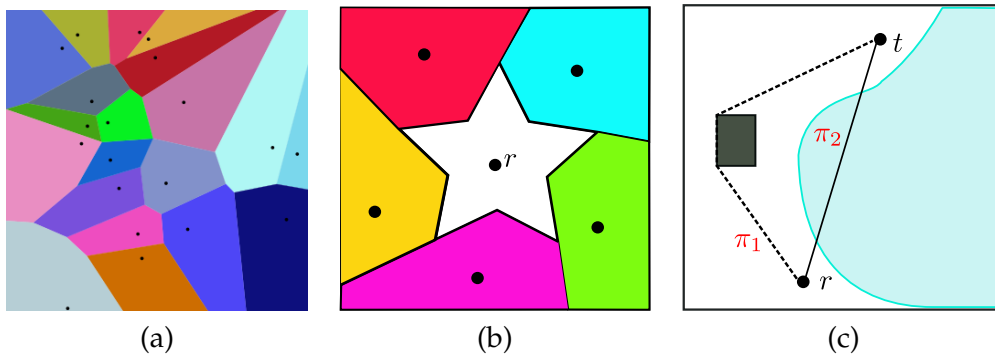
FIGURE 7.1: Different cases of reachability. Each figure represents an example of partitioning with the different subregions distinguished by color. (a): the Voronoi diagram 1 . (b): the central subregion is of star-convex shape with respect to r . (c): the subregion on the left is nonconvex. t can be reached from r by the path \pi_1 which bends around the obstacle and does not pass through the blue area.
