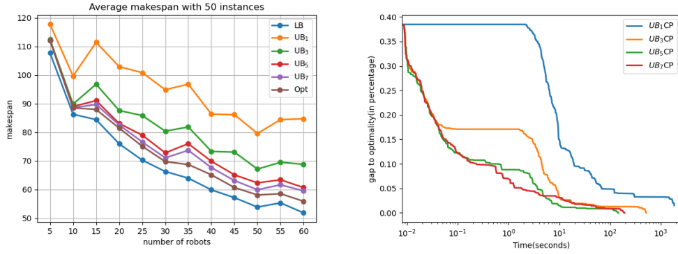
FIGURE 4.2: Left: Evolution of the optimal makespan (Opt), the lower bound (LB) and upper bounds ( UB_i with i \in \{1, 3, 5, 7\} ) when increasing the number n of robots. Right: Evolution of the gap to optimality (in percentage) with respect to time for UB_iCP with i \in \{1, 3, 5, 7\} , on average for the 50 instances with n = 50 robots.
