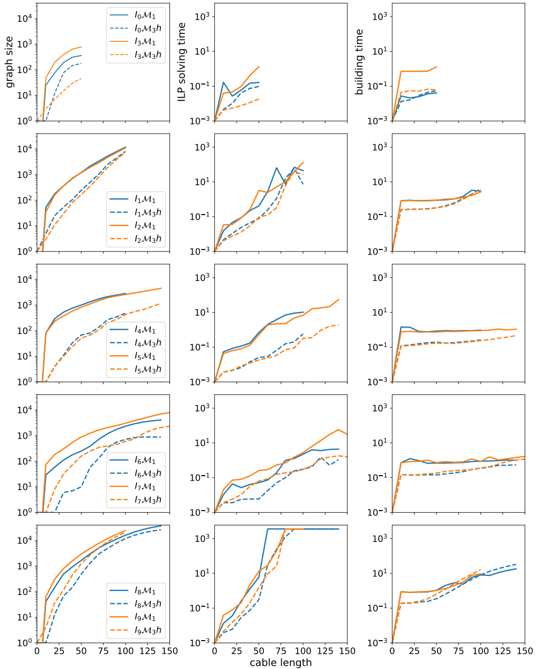
FIGURE 6.16: Evolution of graph sizes and solving times (y-axis with a log scale) with respect to the cable length (x-axis). In each figure, I_x\mathcal{M}_y means the instance I_x solved by model \mathcal{M}_y . First column: the number of vertices in G_{cfg} (model \mathcal{M}_1 ) and G_q (model \mathcal{M}_3h ). Second column: resolution times of the ILP models. Third column: building times of ILP models.
