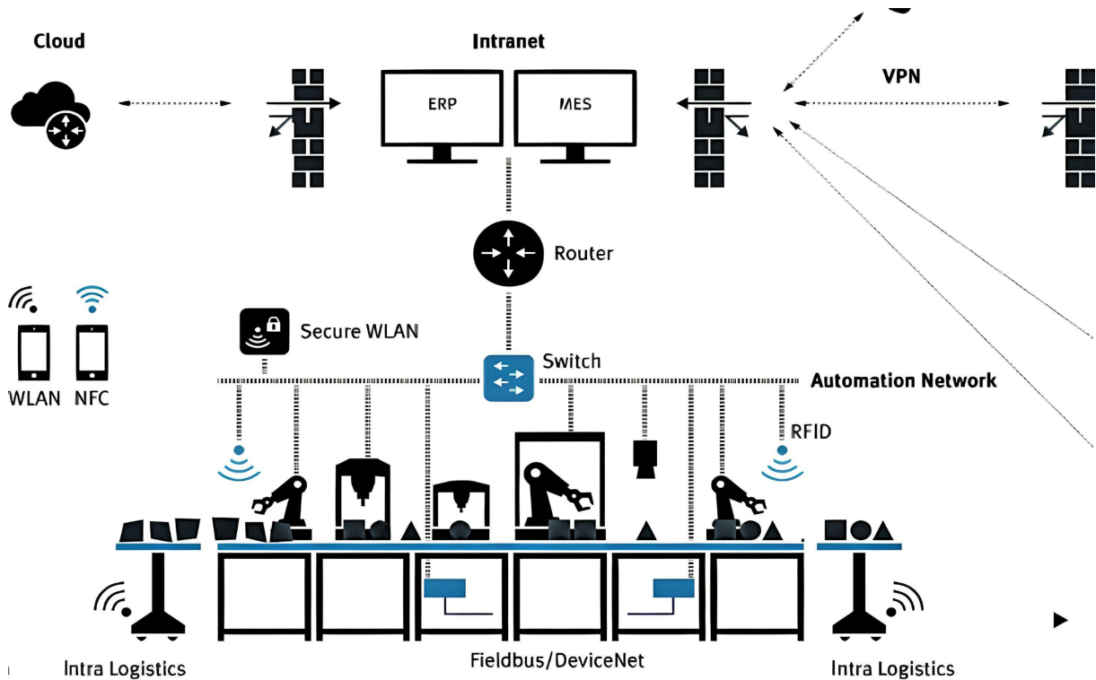
Figure 1.10: LS2N- CPPS schematic view
