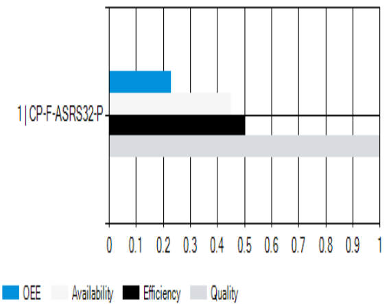
Figure 5.8: Scenario-2 OEE
