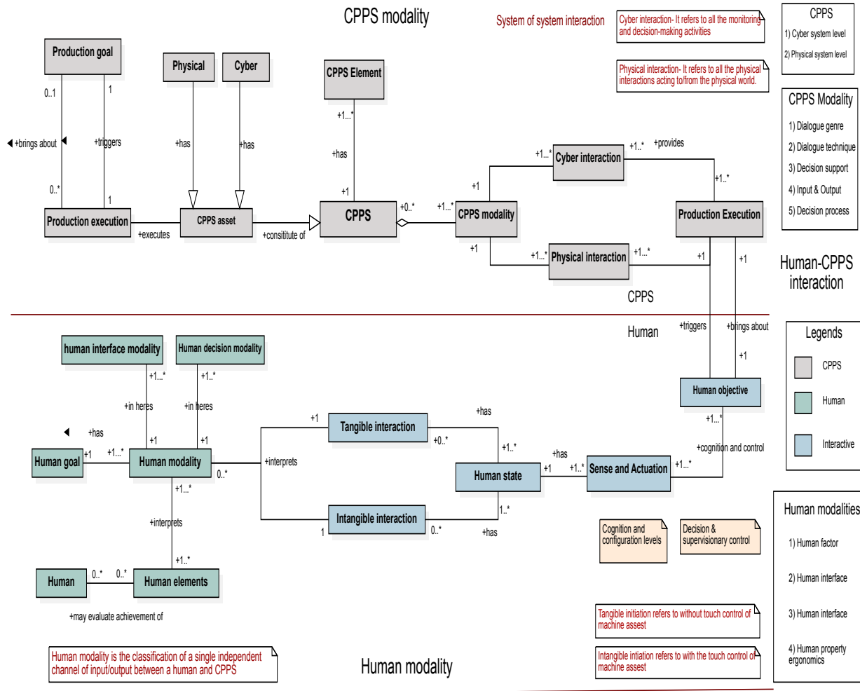
Figure 6.10: Human-CPPS interaction semantics
