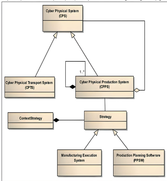
Figure 2.29: CPPS adaptive component [Guarino [1998]]
