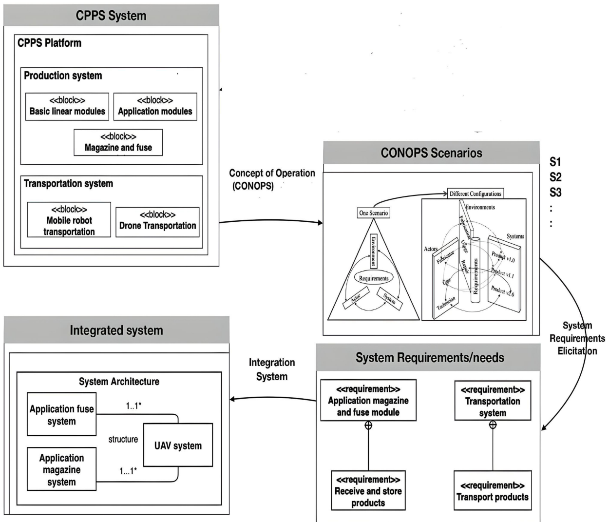
Figure 5.37: Concept of operation(CONOPS)(S1),(S2),(S3)
