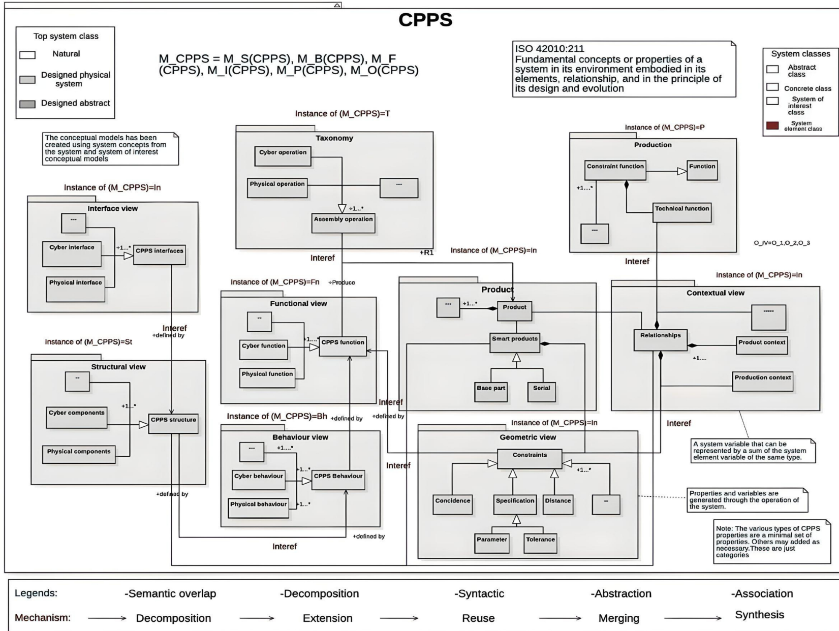
Figure 4.12: CPPS property interrelations views
