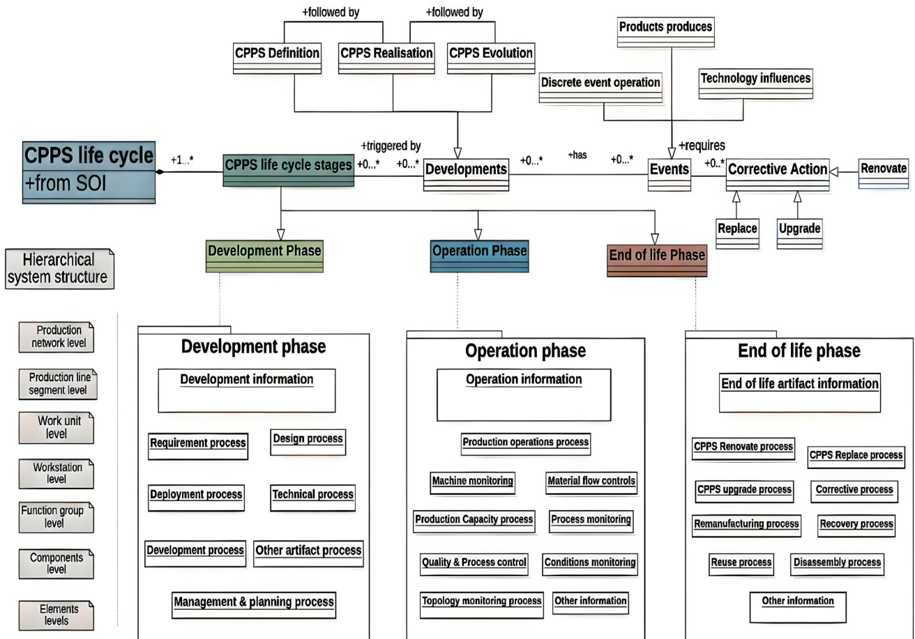
Figure 4.15: CPPS Life-cycle (figure enhanced from [Lüder et al. [2017b]])
