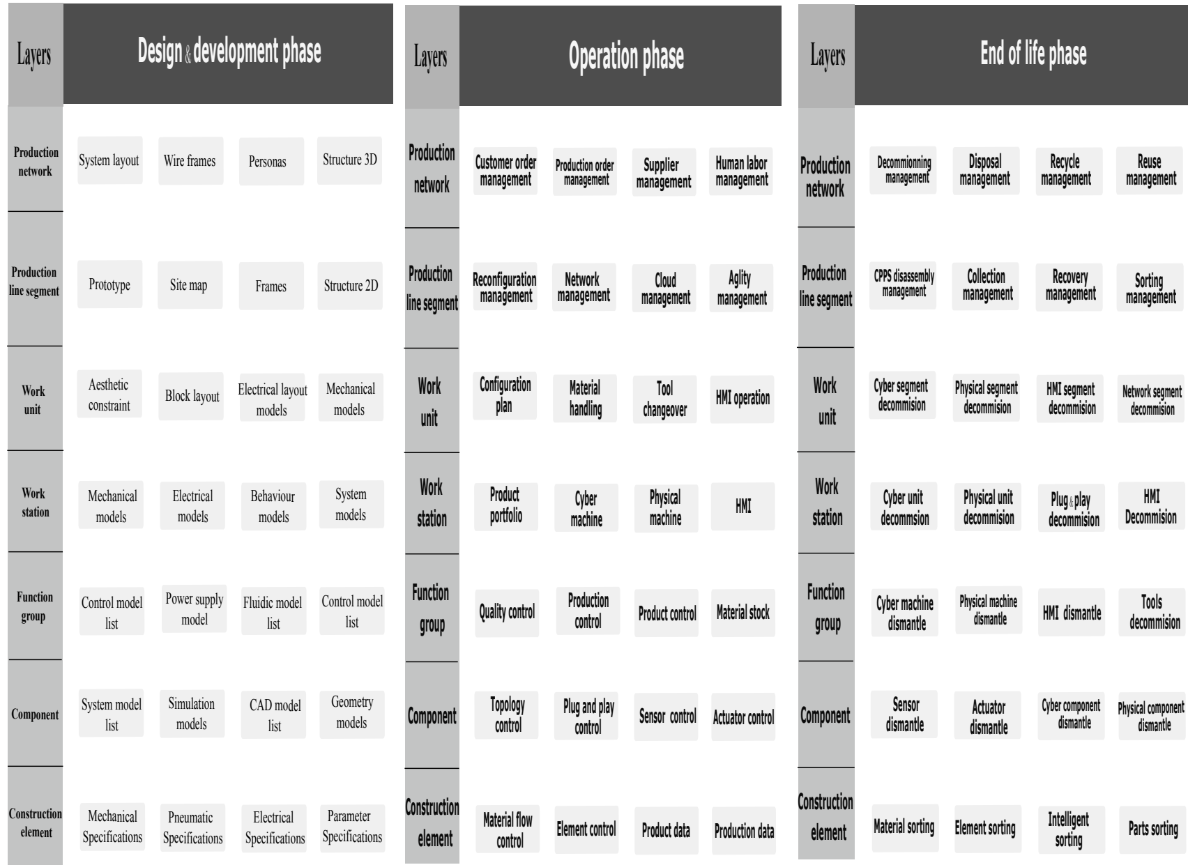
Figure 4.17: CPPS life cycle (figure enhanced from [Lüder et al. [2017b]])
