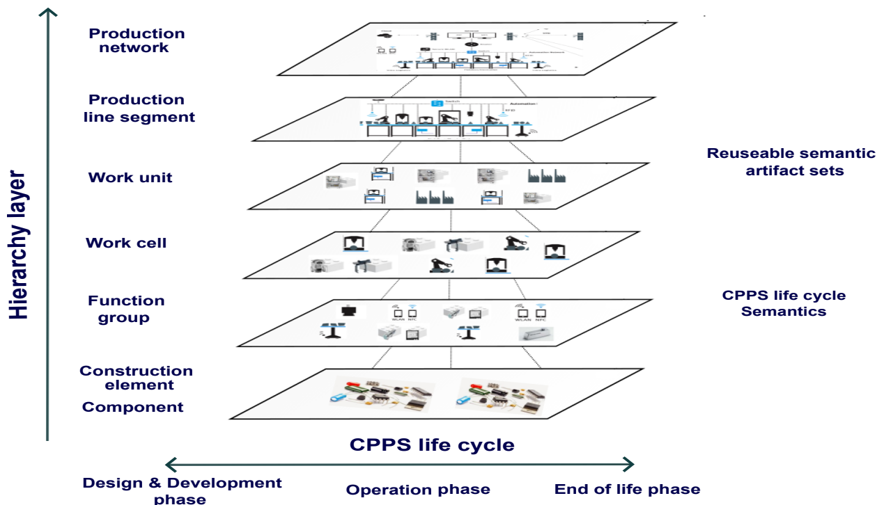
Figure 4.14: CPPS Life-cycle (figure enhanced from [Lüder et al. [2017b]])
