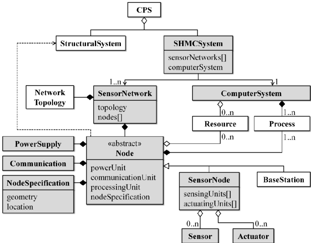
Figure 2.26: CPPS architecture
