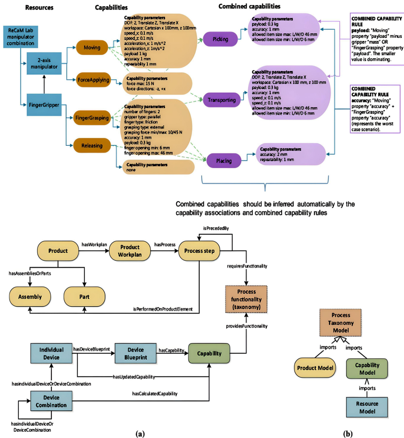
Figure 2.47: Manufacturing system ontology [von Euler-Chelpin [2008]]
