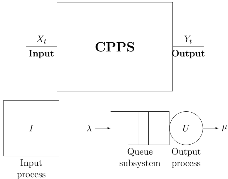
Figure 3.4: CPPS-Input and Output
