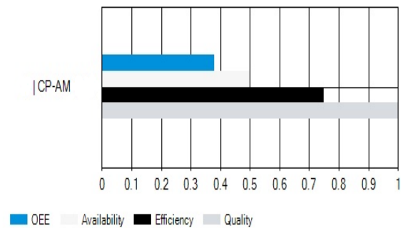
Figure 8.16: Scenario-1 OEE
