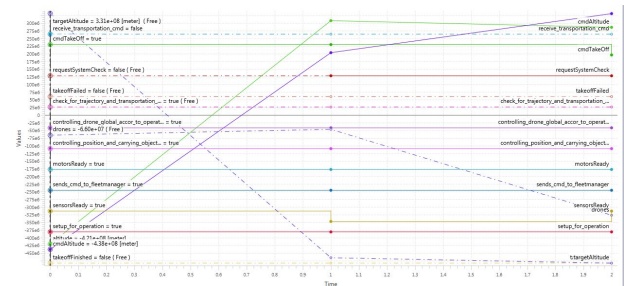
Figure 8.76: Scenario-4-Requirement Obr
