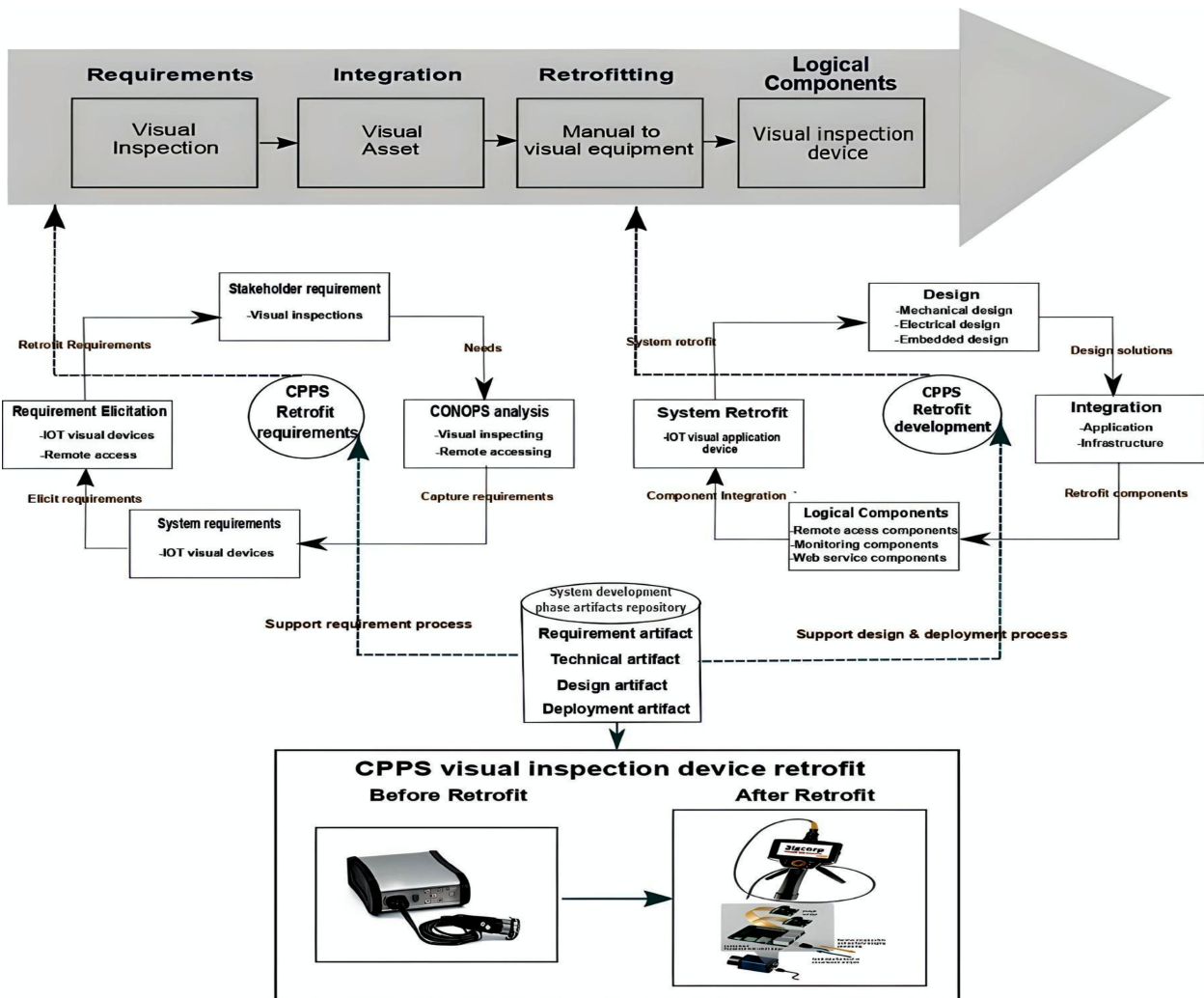
Figure 4.26: Retrofit operation
