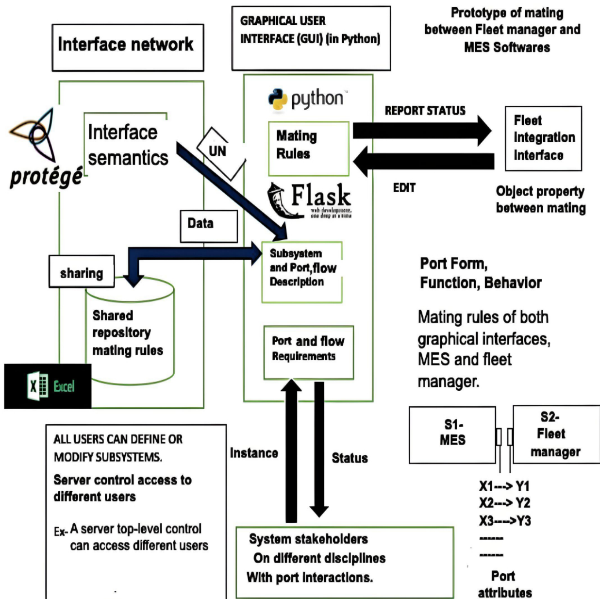
Figure 5.38: Prototype of Collaborative Graphical interface
