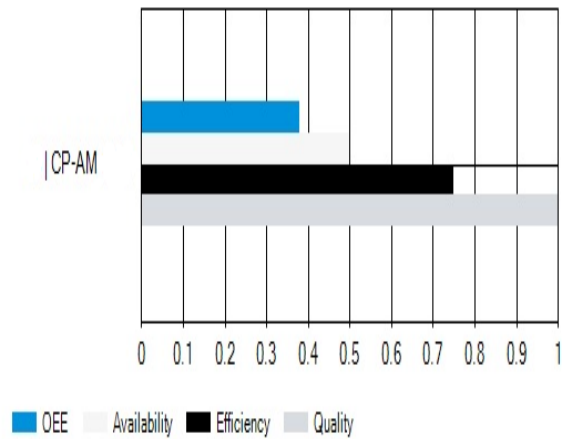
Figure 5.6: Scenario-1 OEE
