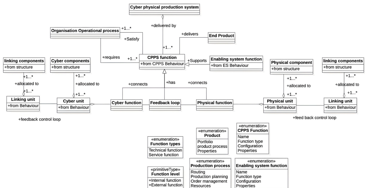
Figure 8.8: CPPS function
