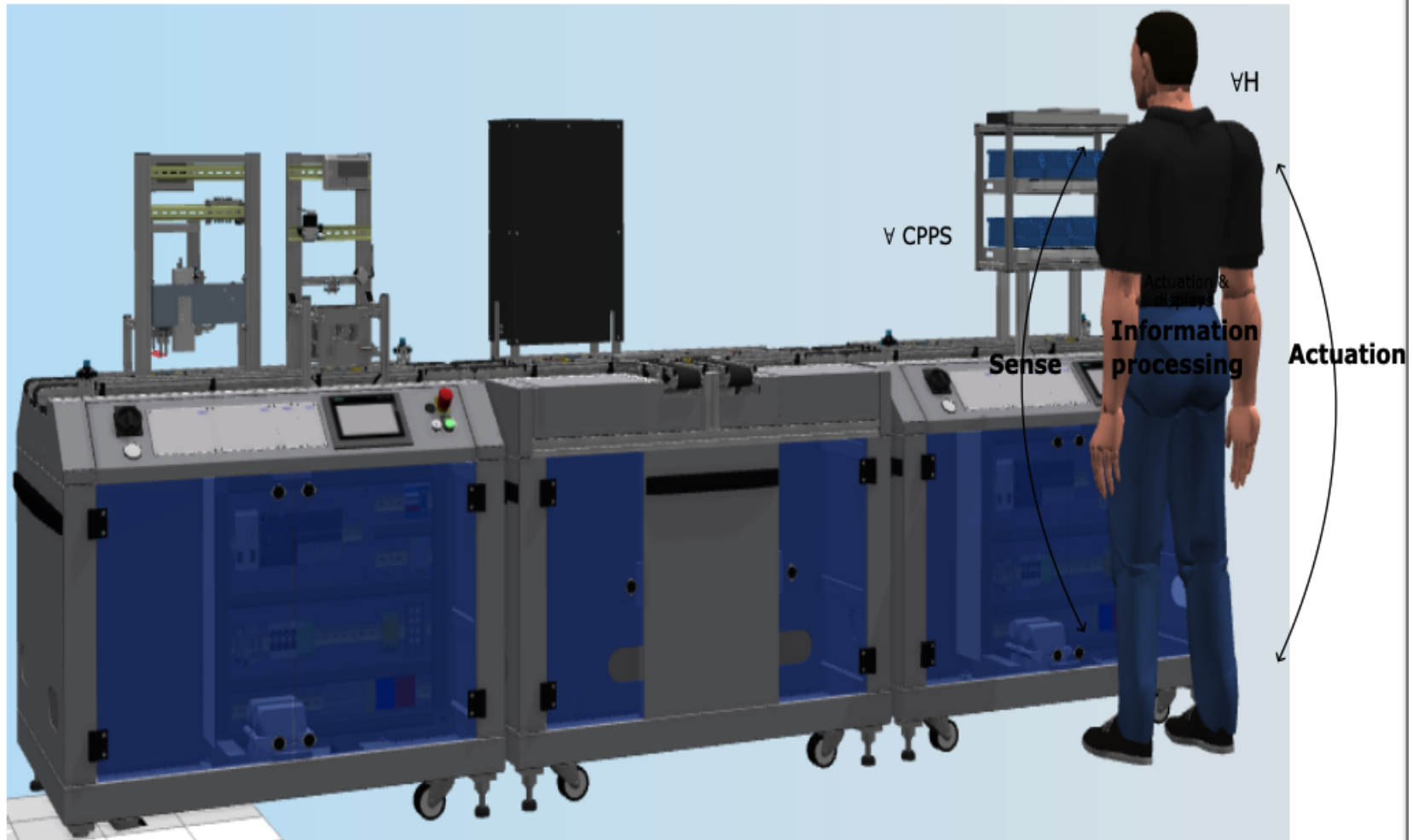
Figure 6.5: Human-CPPS interaction
