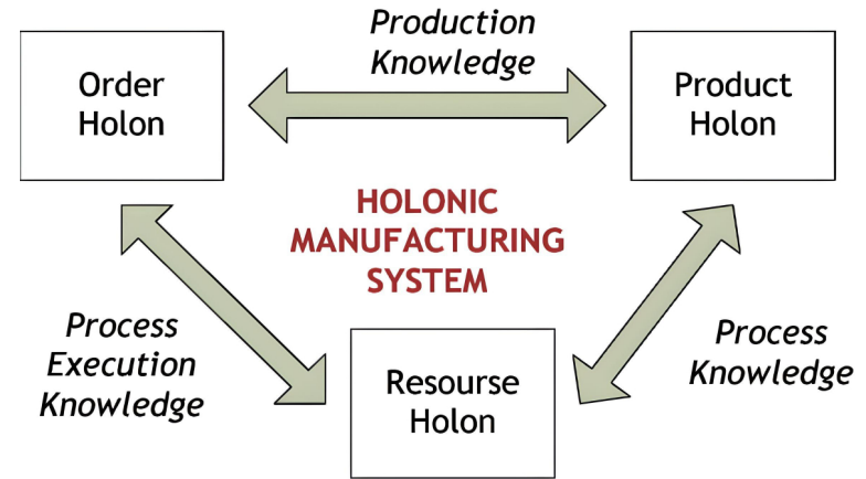
Figure 2.42: holonic manufacturing system [Valckenaers et al. [1997]]
