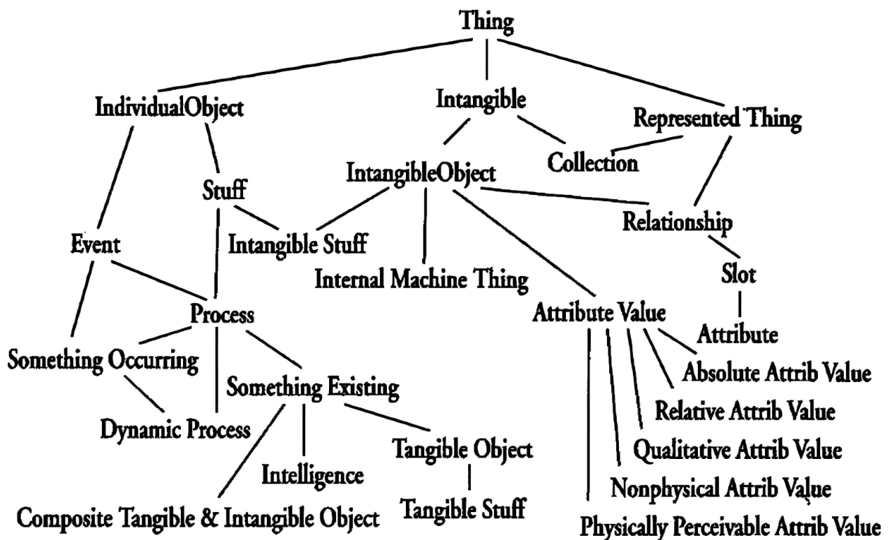
Figure 2.31: Domain ontology [Tazin [2022]]
