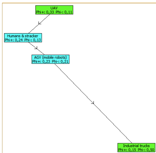
Figure 5.27: PROMETHEE I—Partial Ranking
