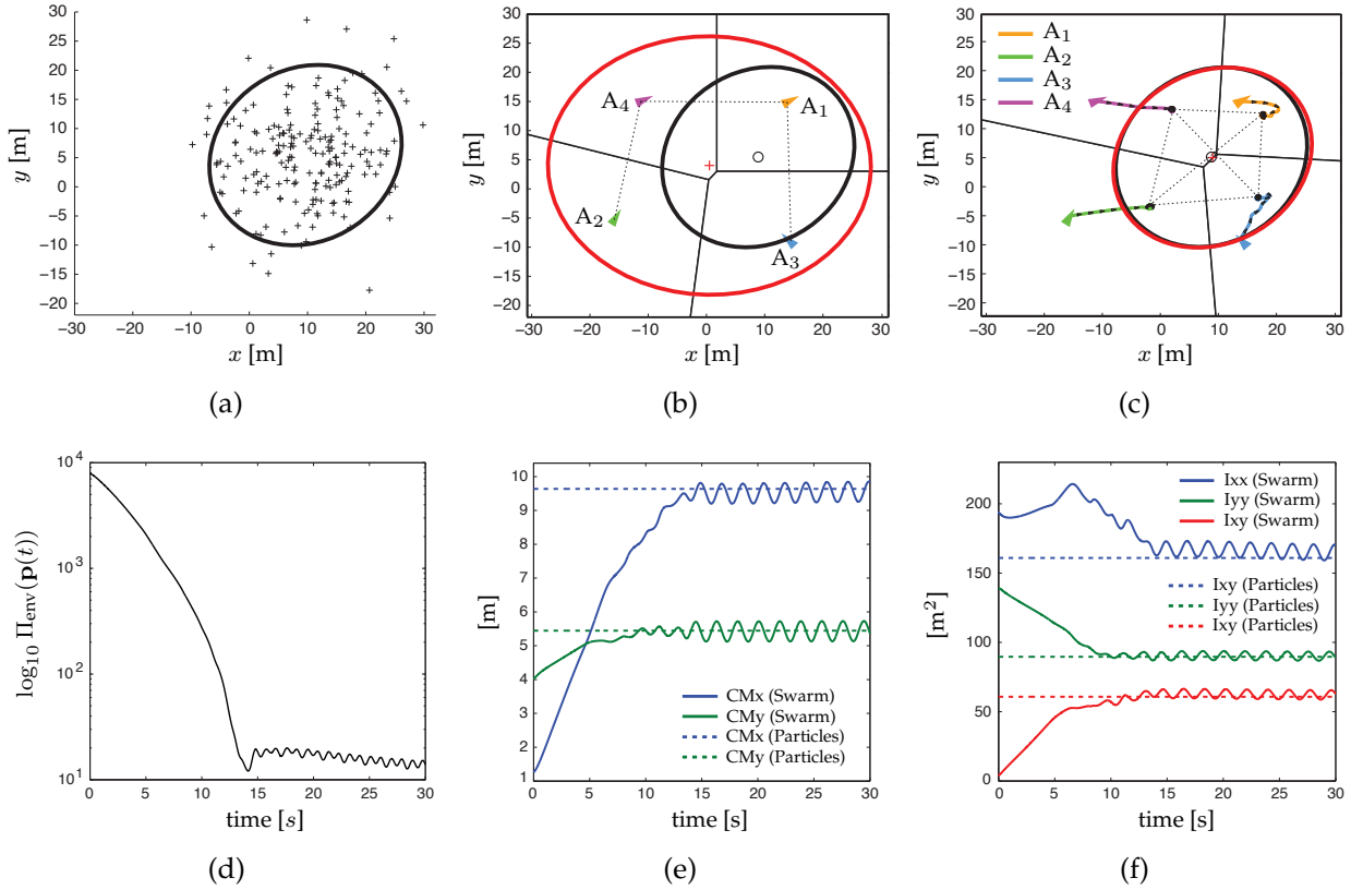
Figure 5.4: Simulation results: (a) Cluster of N = 200 particles and corresponding ellipse of desired geometric moments of the swarm (black); (b) Initial pose of the four agents and corresponding ellipse of geometric moments (red). The initial Voronoi partition of Q and the graph of underlying communication network are represented with solid and dashed lines; (c) Trajectory of the four agents and ellipse of geometric moments at the final time instant (red); (d) Time history of \log_{10} \Pi_{env}(\mathbf{p}(t)) ; (e) First-order moments and (f) second-order moments of \mathbf{f}_{env}^*(t) (dashed, “Particles”) and \mathbf{f}(\mathbf{p}(t)) (solid, “Swarm”).
