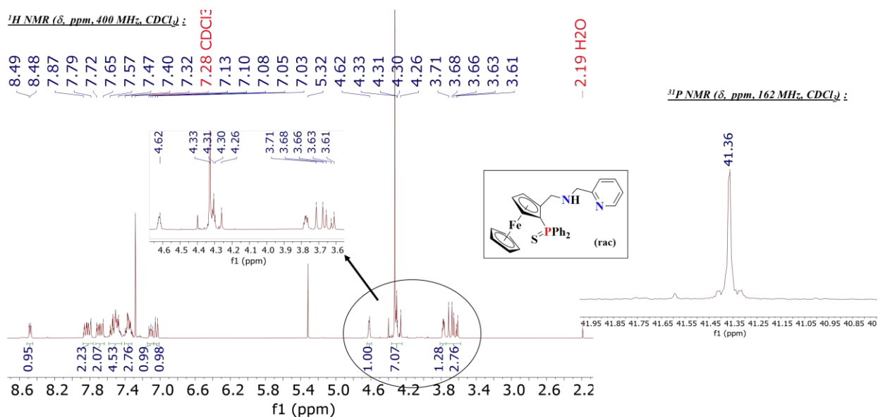
Figure 3. 1: 1 H and 31 P NMR Spectrum (CDCl 3 , 400 MHz) of 3-32
