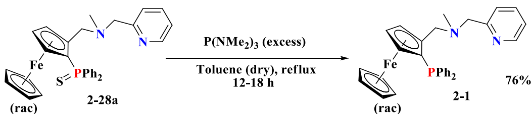
Scheme 2. 16: Phosphine deprotection of ligand 2-28a (R= Me)
