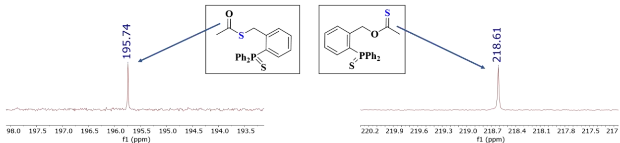
Figure 4. 6: 13 C (CDCl 3 , 125 MHz) NMR spectra (selected region) of 4-46 and 4-47
