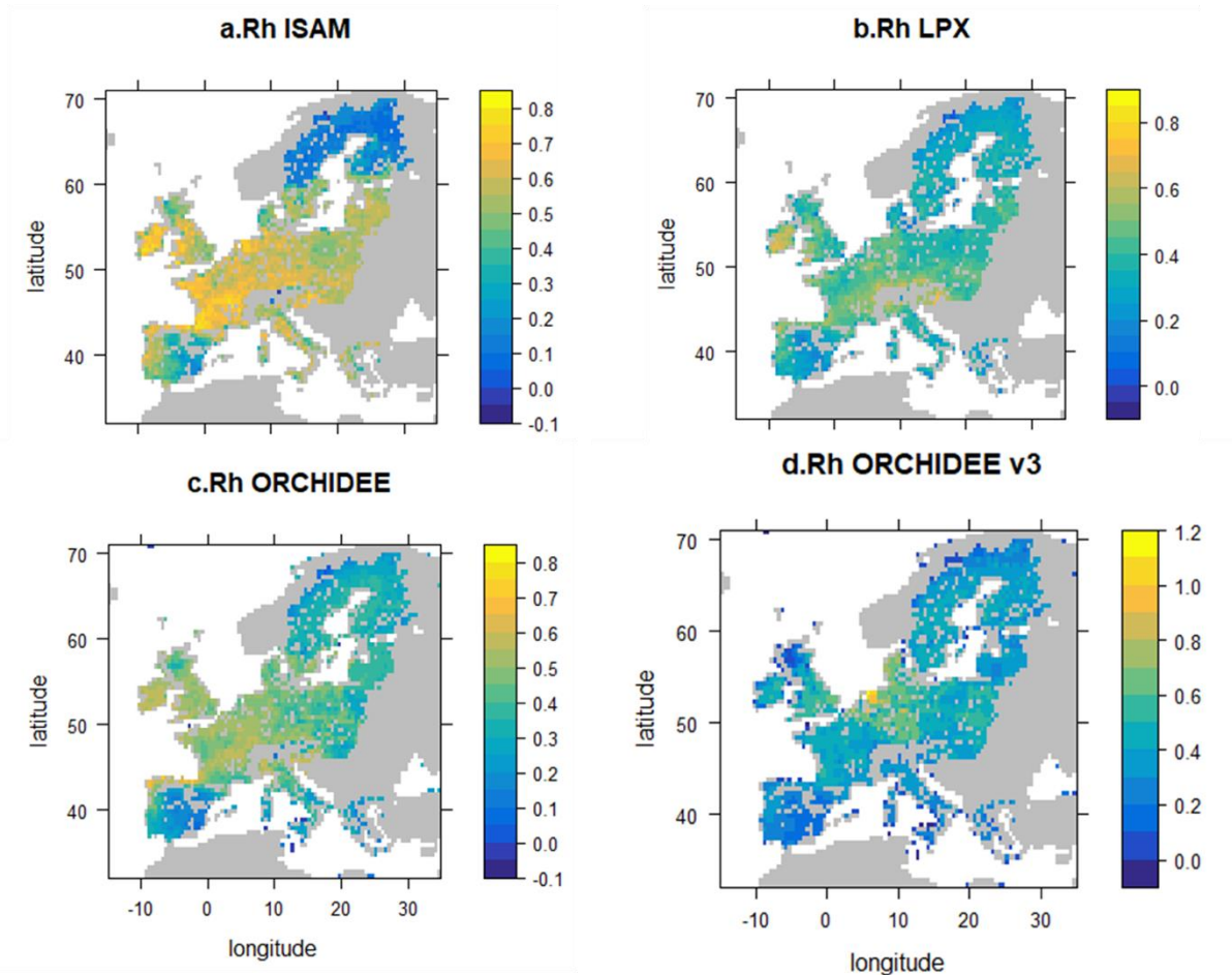
Fig. III.1.2. Heterotrophic respiration (Rh) fluxes from the different LSM models in kgC m -2 year -1 . a. ISAM model, b. LPX model, c. ORCHIDEE model, d. ORCHIDEE v3 model filtered over the EU territory.
