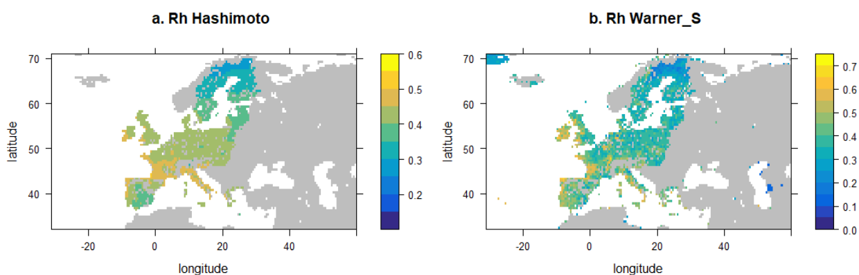
Fig. III.1.1. Heterotrophic respiration (Rh) fluxes from the observations products in kgC m -2 year -1 . a. Rh Hashimoto, b. Rh Warner_S filtered over the EU territory.
