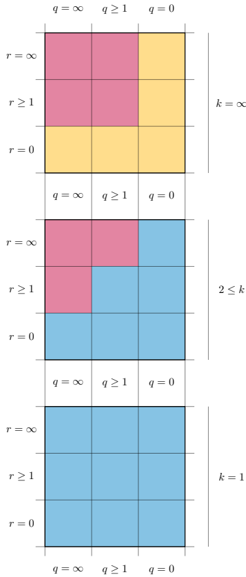
Figure 4.13. The preservation cube: studying whether formulas preserved under \Rightarrow_q^{r,k} are equivalent over \text{Fin}(\sigma) to existential local sentences. In red, the answer is ‘NO’, in blue, the answer is ‘YES’. In yellow, the answer is ‘YES’, but the proof is postponed to Chapter 5 (A Local-to-Global Preservation Theorem).
