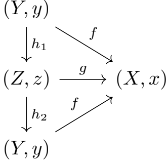
Figure 8.1.: Since f and g are transitive objects of \text{Elt}(F)/(X, x) , there exists functions h_1, h_2 such that the above diagram commutes in \text{Elt}(F) .
