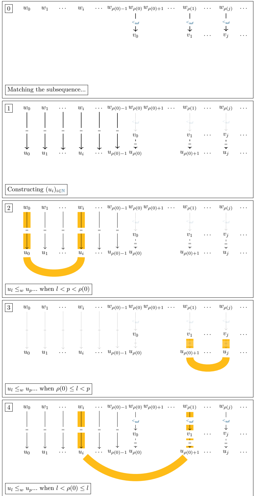
Figure 7.6.: Illustration of the merging process in Higman’s Lemma.
