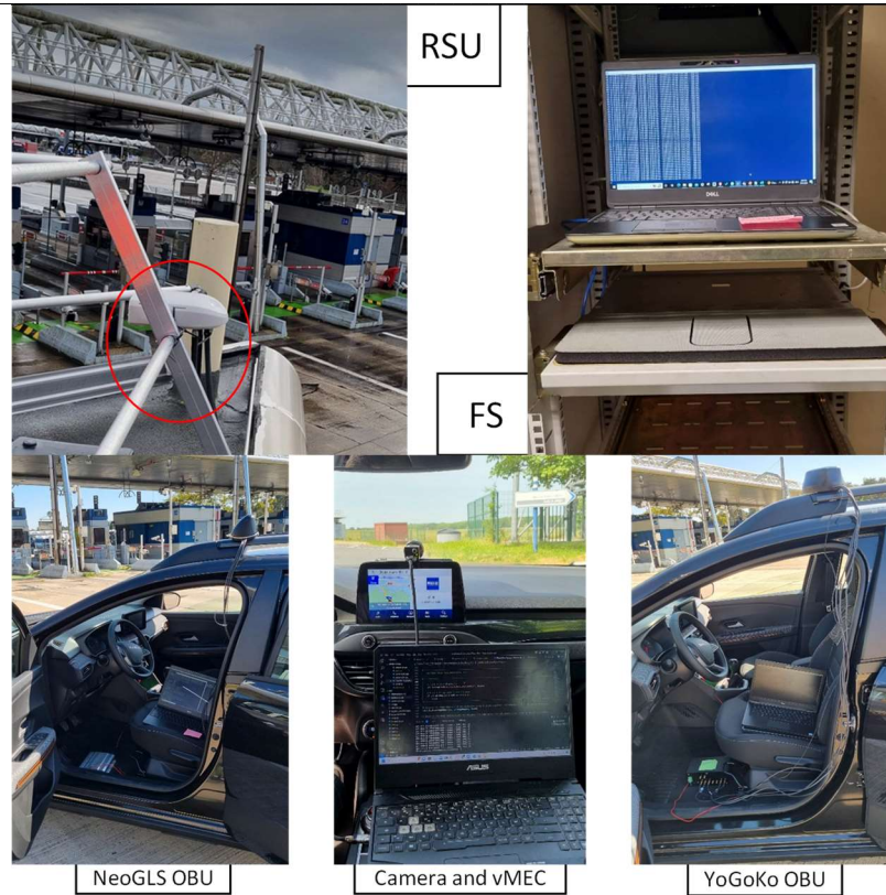
Figure 5.6. Used equipment
