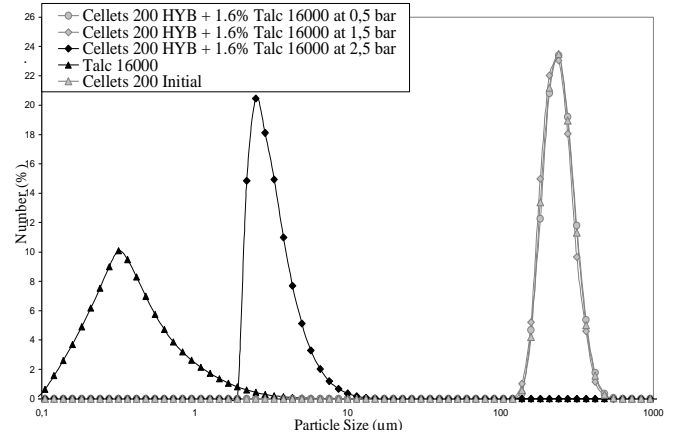
Figure IV.99. Number Particle Size Distribution of 1.6 % Talc 16000 Coated Pre-treated Cellets 200 Particles in Turbula
