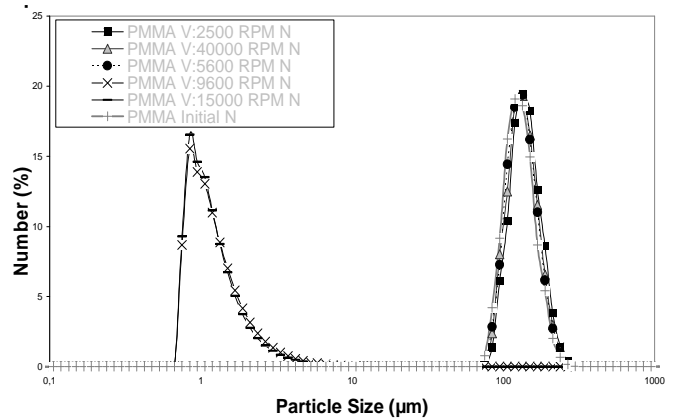
Figure III.5. Number Particle Size Distribution of PMMA Particles Before and After Treatment with Different RPM Operating Velocities
