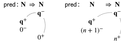
Figure 4.6: Strategy for pred
