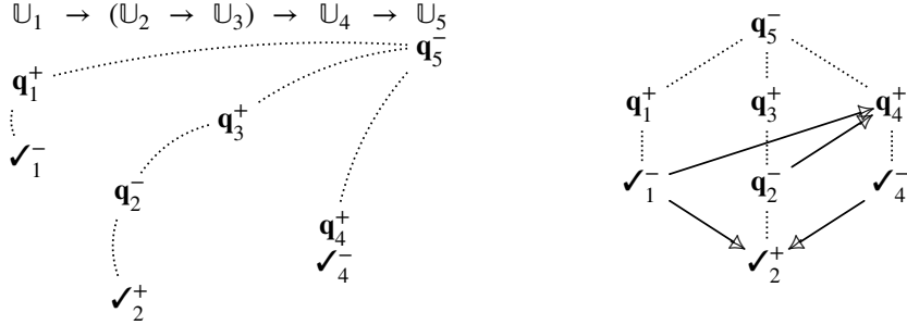
Figure 5.9: Example of definability of plays in IA_{//}
