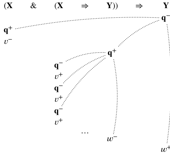
Figure 4.7: Typical plays for \text{let}_{X,Y}
