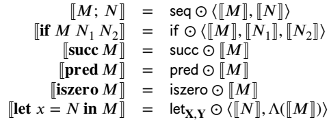
Figure 4.5: Basic interpretation clauses
