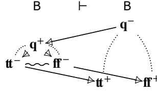
Figure 10.2: Deterministic copycat
