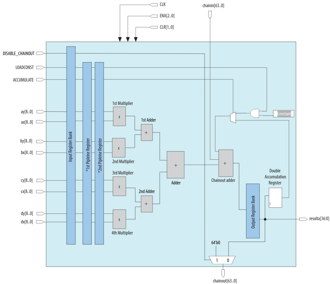
*This block diagram shows the functional representation of the DSP block. The pipeline registers are embedded within the various circuits of the DSP block.
