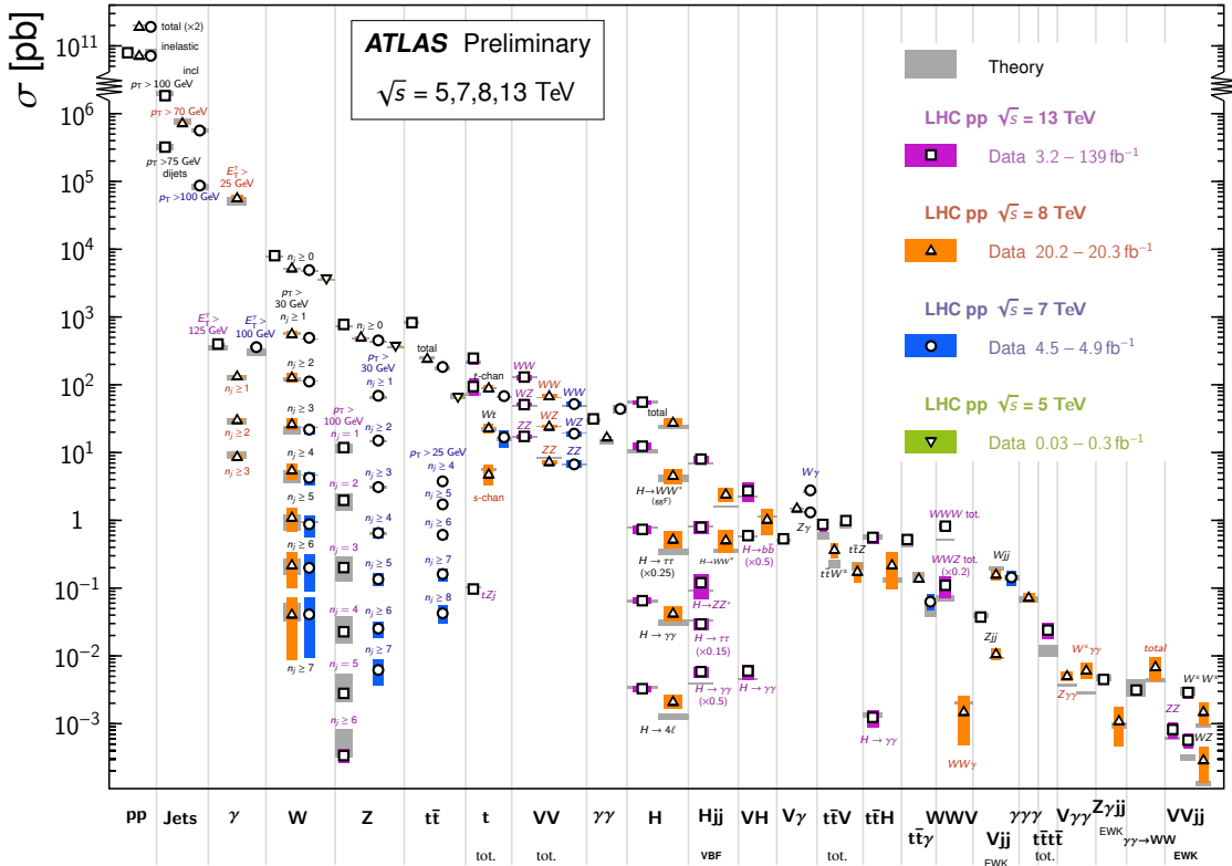
Figure 2: Summary of several Standard Model total and fiducial production cross-section measurements [48]. The measurements are corrected for branching fractions and compared to the corresponding theoretical predictions.
