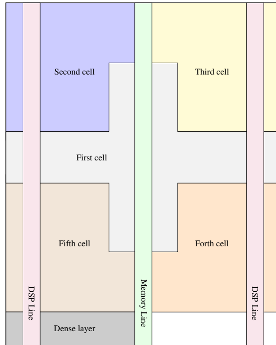
Figure 3.33: Schematic view of the optimised placement of the Vanilla RNN showing the 5 cells and the dense layer with respect to the memory and DSP lines inside the FPGA.
