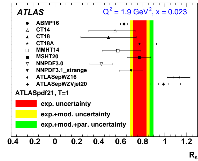
Figure 1.12: R_s = s(s+\bar{s})/x(\bar{u}+\bar{d}) at x = 0.023 and Q^2 = 1.9 \text{ GeV}^2 from the ATLASpdf21 set [130] compared to the ABMP16 [131], CT14 [132], CT18, CT18A [133], MMHT14 [134], MSHT20 [135], NNPDF3.0 [136], NNPDF3.1_strange [137], ATLASepWZ16 [53], and ATLASepWZV-jets20 [138] sets.
