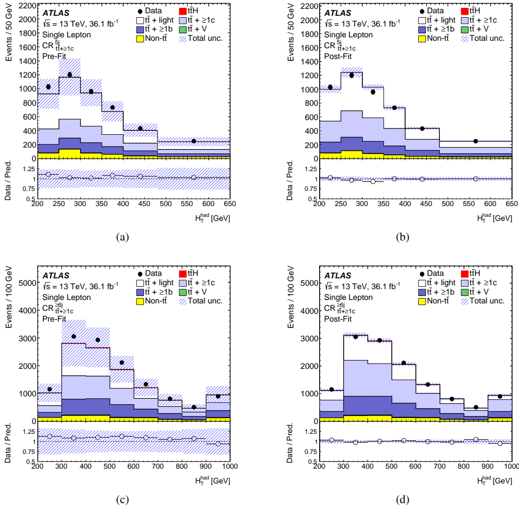
Figure 2.8: Comparison between data and prediction for the H_T^{\text{had}} distributions in the single-lepton t\bar{t} + \geq 1c -enriched control regions (a, c) before, and (b, d) after the combined dilepton and single-lepton fit to the data. Despite its small contribution in these control regions, the t\bar{t}H signal prediction is shown stacked at the top of the background prediction, normalized to the SM cross-section before the fit and to the fitted \mu after the fit. The pre-fit plots do not include an uncertainty for the t\bar{t} + \geq 1b or t\bar{t} + \geq 1c normalization.
