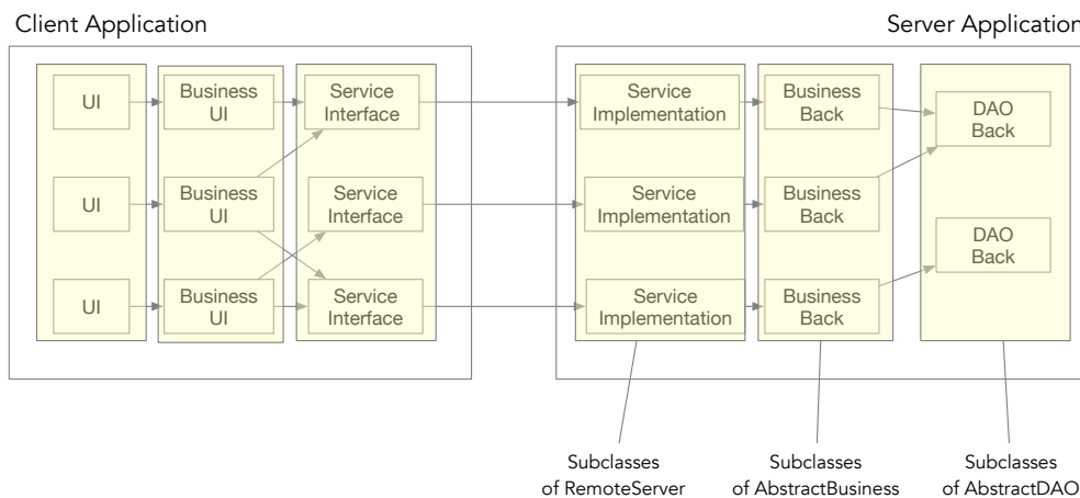
Figure 3.1: A Typical example of the Client-Server Architecture layers
