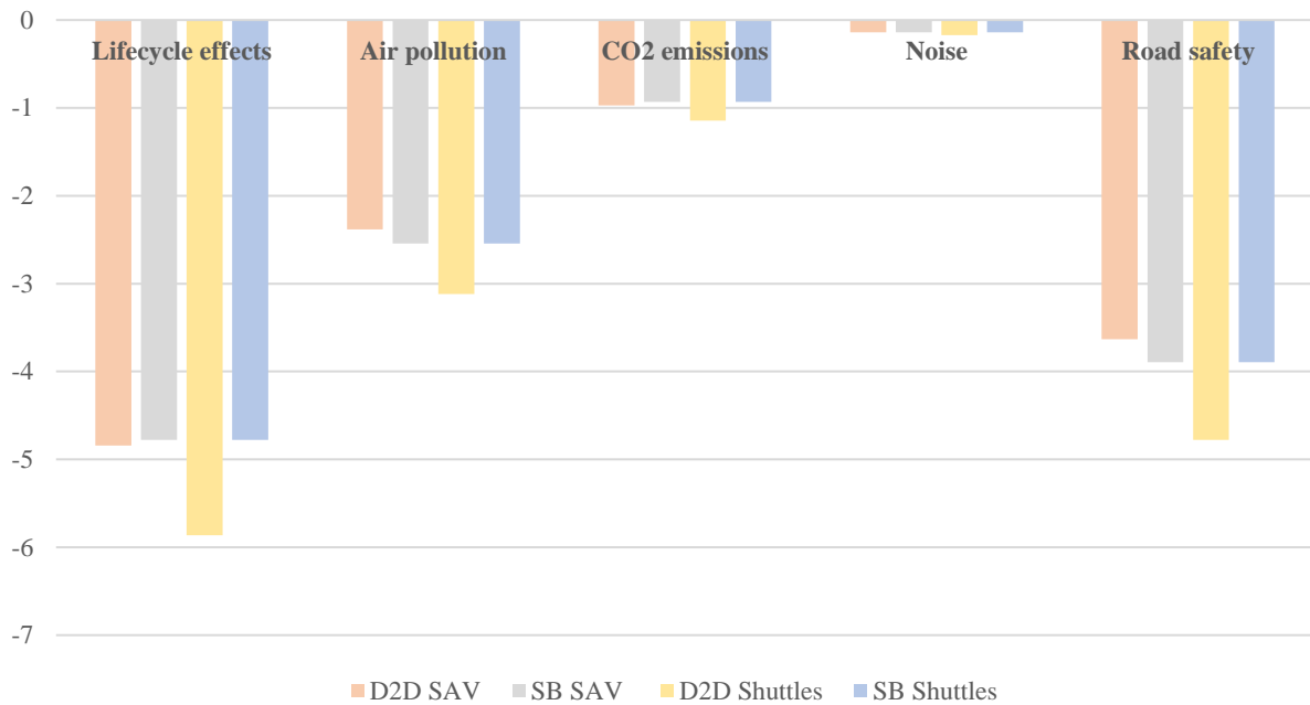
Figure 68. Externalities impact
