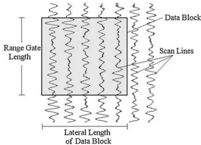
Figure 3.5: Diagram showing the time-gated RF lines contained within one ROI (data Block) Reproduced from Mamou et al. [24]
