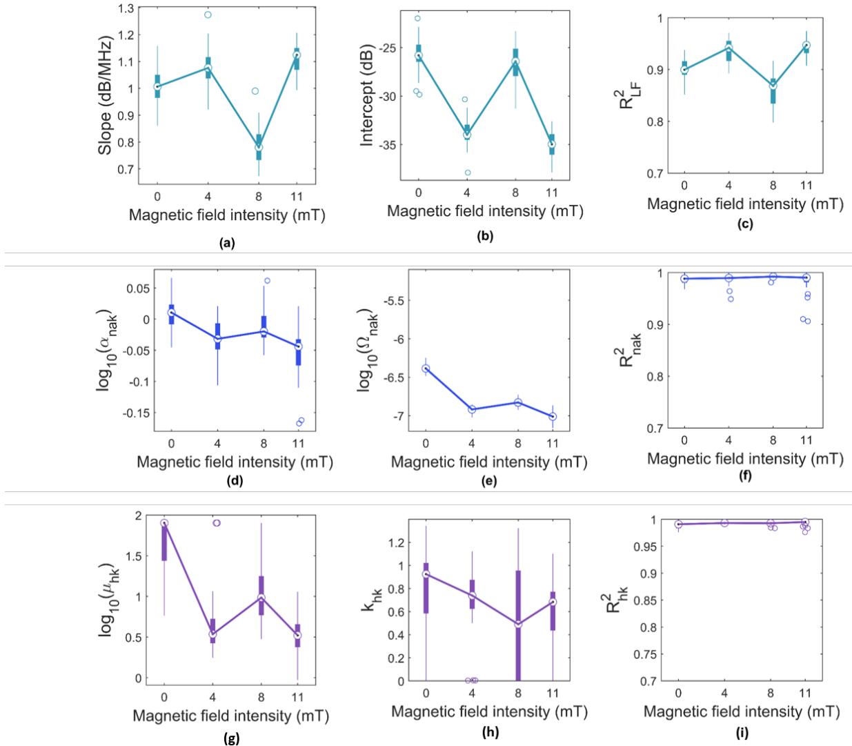
Figure 8.8: Vertical steady-state experiment results. The first row shows the Lizzi-Feleppa parameters versus magnetic field intensity, the second row shows the Nakagami parameters and the third row the Homodyned-K parameters. (a) BSC slope (b) BSC intercept. (c) Goodness of the BSC linear fit. (d) Nakagami parameters \alpha_{nak} . (e) Scaling factors \Omega_{nak} . (f) The goodness of fit R_{nak}^2 for Nakagami distributions. (g) Scatterer clustering parameter \mu_{hk} . (h) Coherent to diffuse signal ratio k_{hk} . (i) The goodness of fit R_{hk}^2 for Homodyned-K distributions. The coefficients \alpha_{nak} , \Omega_{nak} and \mu_{hk} underwent compression using a base-10 logarithm due to their extensive value range.
