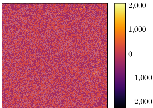
(a) G^2
