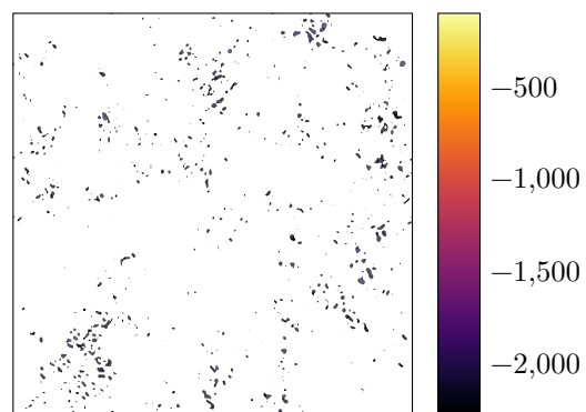
(b) G^2 < \langle G^2 \rangle_\Omega - 2\sigma(G^2)
