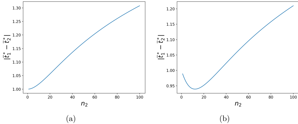
Fig. A3.10: Influence of the density of species 2 n_2 on the phenotypic distances between the two species, when (a) predation is low compared to reproductive interference and (b) when predation is high compared to reproductive interference, assuming strong female and predator discriminations. Simulations were run assuming: (a) d = 0.02 or (b) d = 0.05 . The default parameters values are as follows: G_{t_1} = G_{p_1} = 0.01 , a_1 = 1 , c_{RI} = 0.01 , b = 1 , \lambda_1 = 0.1 , \lambda_2 = 0.1 , n_1 = 10 , n_2 = 20 , s_1 = 0.0025 , t_{a1} = 0 and t_{a2} = 1 .
