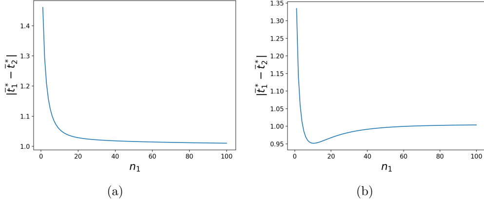
Fig. A3.7: Influence of the density of species 1 n_1 on the phenotypic distances between the two species, when (a) predation is low compared to reproductive interference and (b) when predation is high compared to reproductive interference, assuming strong female and predator discriminations. Simulations were run assuming: (a) d = 0.02 or (b) d = 0.05 . The default parameters values are as follows: G_{t_1} = G_{p_1} = 0.01 , a_1 = 1 , c_{RI} = 0.01 , b = 1 , \lambda_1 = 0.1 , \lambda_2 = 0.1 , n_1 = 10 , n_2 = 20 , s_1 = 0.0025 , t_{a1} = 0 and t_{a2} = 1 .
