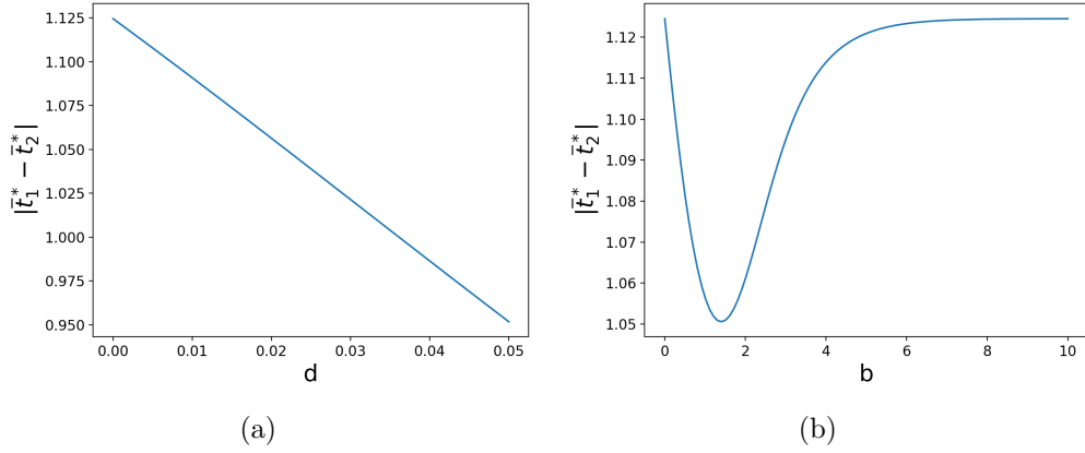
Fig. A3.5: Influence of the strength of predation d (a) and of predator discrimination b (b) on the phenotypic distances between the two species, assuming strong female and predator discriminations. The default parameters values are as follows: G_{t_1} = G_{p_1} = 0.01 , a_1 = 1 , c_{RI} = 0.01 , b = 1 , d = 0.02 , \lambda_1 = 0.1 , \lambda_2 = 0.1 , n_1 = 10 , n_2 = 20 , s_1 = 0.0025 , t_{a1} = 0 and t_{a2} = 1 .
