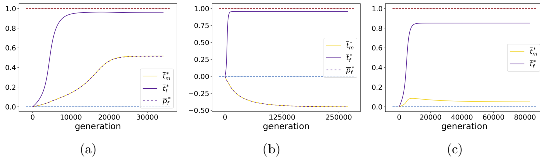
Fig. A4.5: Evolution of the mean male trait and female trait and preference values across generations (a)(b) when reproductive interference or (c) sexually contrasted predation promotes sexual dimorphism. We assume: (a) c_{RI} = 0.01 , a = 10 , s = 0.0025 , d_m = 0.05 , (b) c_{RI} = 0.01 , a = 2.5 , s = 0.0025 , d_m = d_f = 0.05 (c) c_{RI} = 0 , a = 0 , s = 0.01 , d_m = 0.005 . We assume for the other parameters: G_{t_m} = G_{t_f} = G_{p_f} = 0.01 , G_{t_m t_f} = 0.001 , c = 0.1 , b = 5 , d_f = 0.05 , \lambda = 0 , N = 100 , \lambda' = 0.01 , N' = 200 , t_a = 0 , \bar{t}' = 1 . The curves stop when the male trait and female trait and preference values reach equilibrium.
