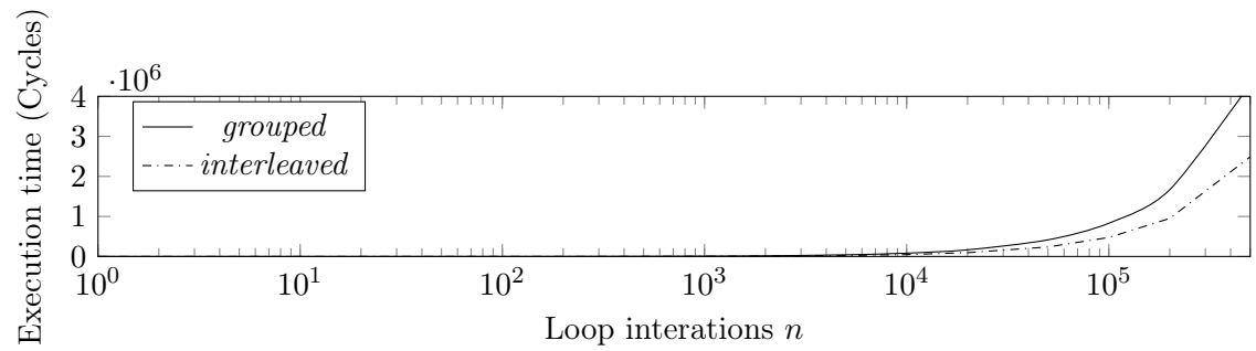
(a) Execution time of the experiments depending on the number of loop iterations n .
