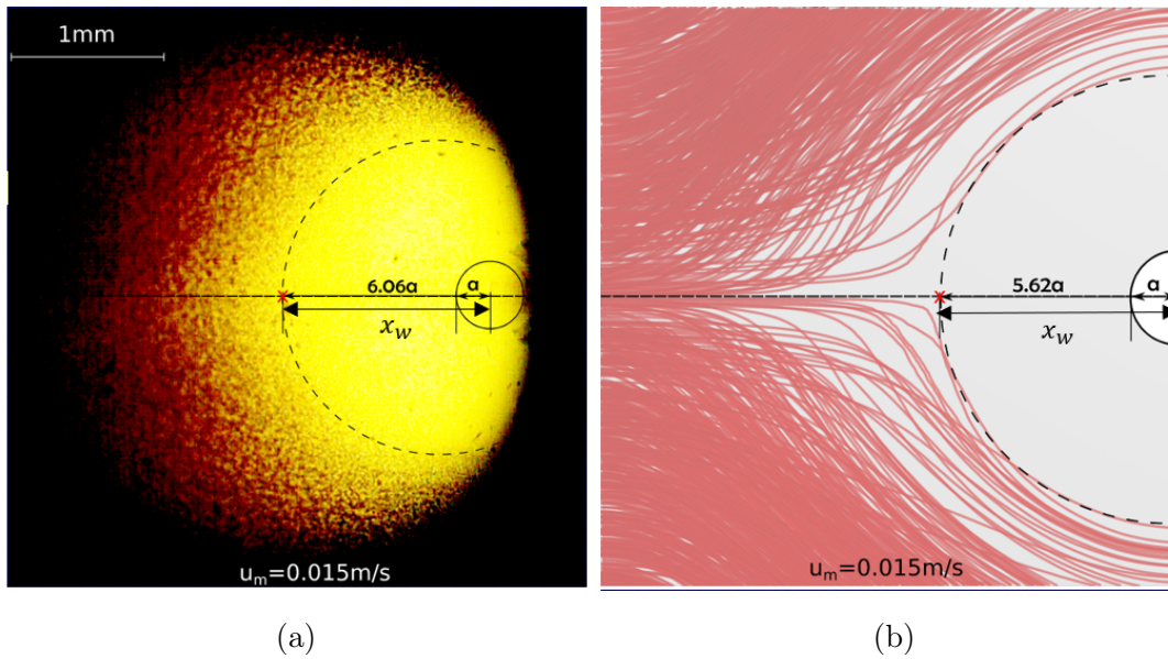
Figure 4.2: Distributions of water droplets in oil at the inlet of an EHL contact and estimation of inlet distance with characteristic droplet diameter of 8\ \mu\text{m} with (a) experimental observations at 0.015\ \text{m/s} , (b) numerical results at 0.015\ \text{m/s}
