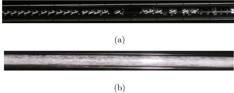
Figure 1.10: Flow patterns of the ester oil ISO VG10l-refrigerant R134a mixture flowing through a straight horizontal tube: (a) bubbly flow and (b) foam flow from Ref. [82]
