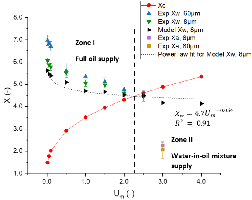
Figure 4.3: Comparison between water droplets position obtained experimentally and numerically for droplet size of 8 \mu m and 60 \mu m and critical position of starved condition on the central line. With X_c the critical position of starved condition, X_w the closest position of water droplets and X_a the closest position influenced by air-oil meniscus to the contact area.
