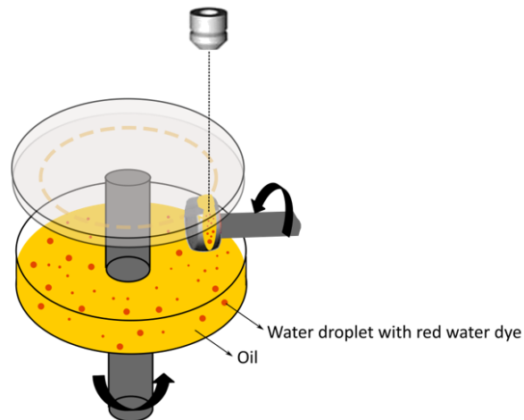
Figure 2.8: Schematic diagram of the ball-on-disc test rig.
