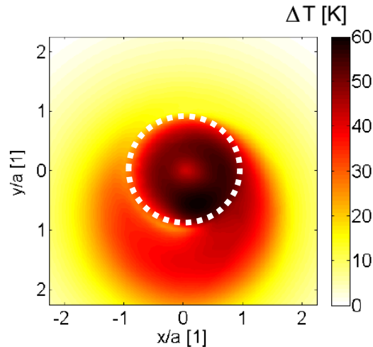
Figure 1.7. Temperature rise of a high spinning contact and its surrounding at the lubricant/upper solid boundary, from [7]. The contact area is marked with a dotted circle.
