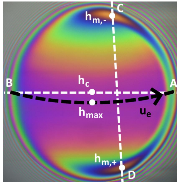
Figure 4.1. Representative film thicknesses in a spinning contact (interferogram extracted from [7]). The center of rotation of the specimen is found above the image.
