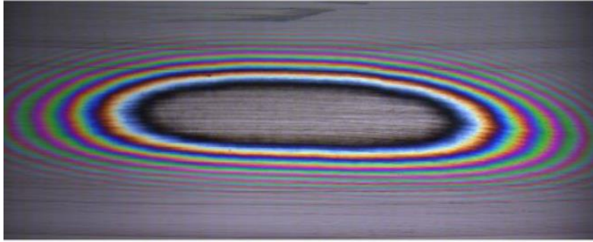
Figure 1.8. Interferogram of a banana-shaped contact created by a toroidal-end specimen and a disk, from [1].
