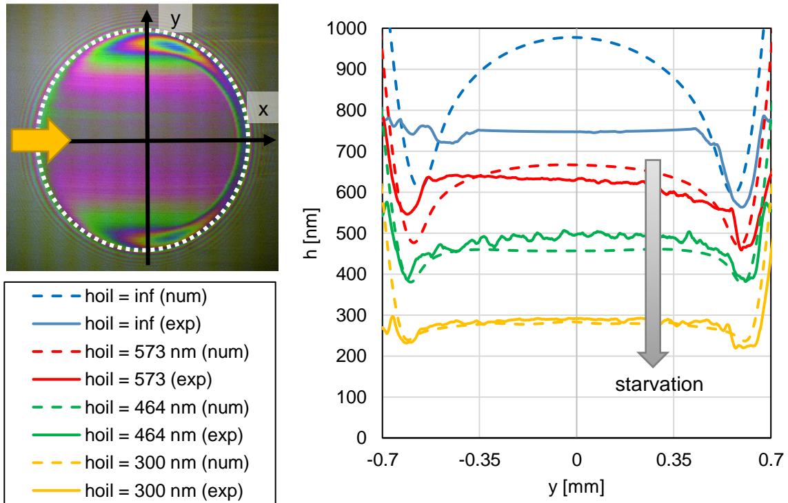
Figure 3.12. Film thickness along the y-axis for u_e = 0.50 \text{ m/s} and w = 400 \text{ N} . The direction of the entrainment velocity is represented by a yellow arrow. The interferogram (left) corresponds to the fully flooded case. The Hertzian contact area is marked by a dotted circle.
