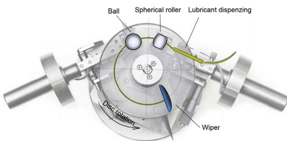
Figure 2.3. Overview of a modified test rig for starved contacts (extracted from [46]).
