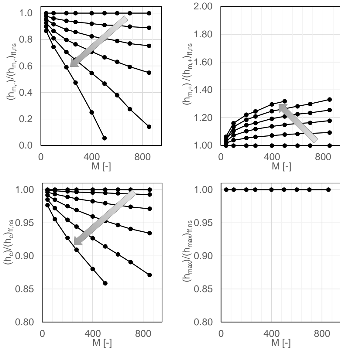
Figure 4.3. Variation of the representative film thicknesses with respect to the dimensionless number M and various spin rotation velocities, with L = 6.6 . An arrow indicates the direction of increasing spin value, in steps of 1000 rad/s.
