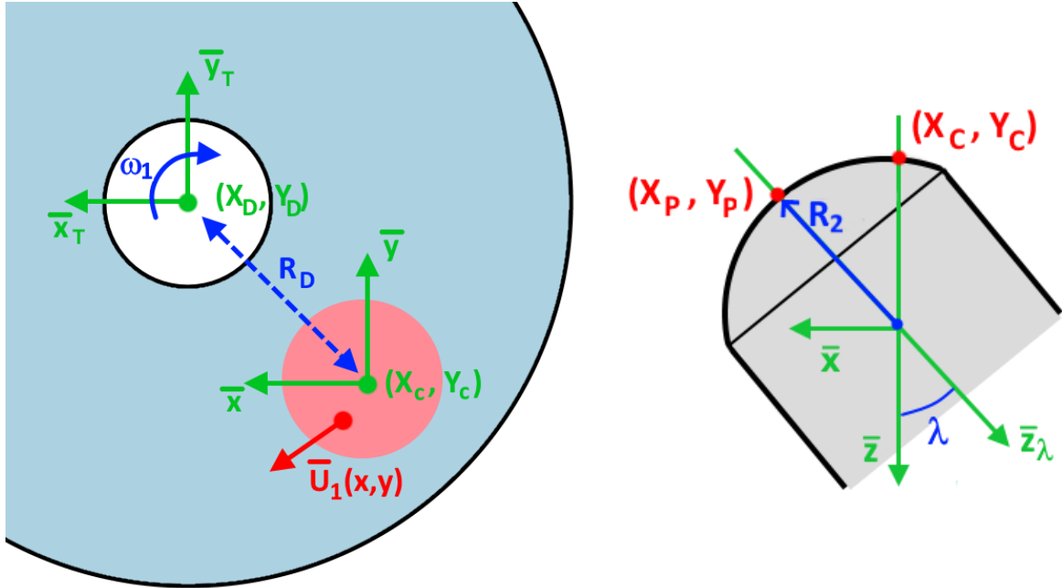
Figure 2.6. Left: top view of a contact between a disk and a spherical end specimen. Right: detail of the spherical-end specimen head. \bar{z}_\lambda is the axis of rotation of the specimen, R_2 is its curvature radius and \lambda the spin angle.
