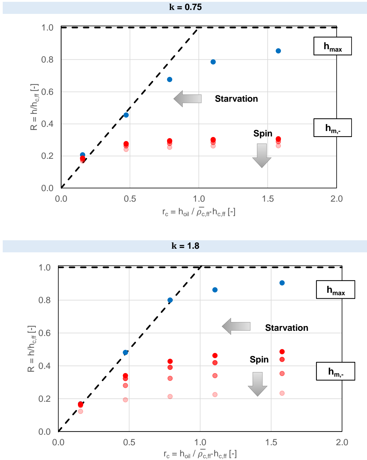
Figure 4.14. Dimensionless maximum ( R_{max} ) and critical minimum ( R_{m,-} ) film thickness variations with respect to the dimensionless oil supply ( r_c ) for different spin velocities ( u_e = 2 m/s, w = 800 N, T = 30^\circ\text{C} , R_x = 80 mm) and to ellipticities: k = 0.75 (above) and k = 1.8 (below).
