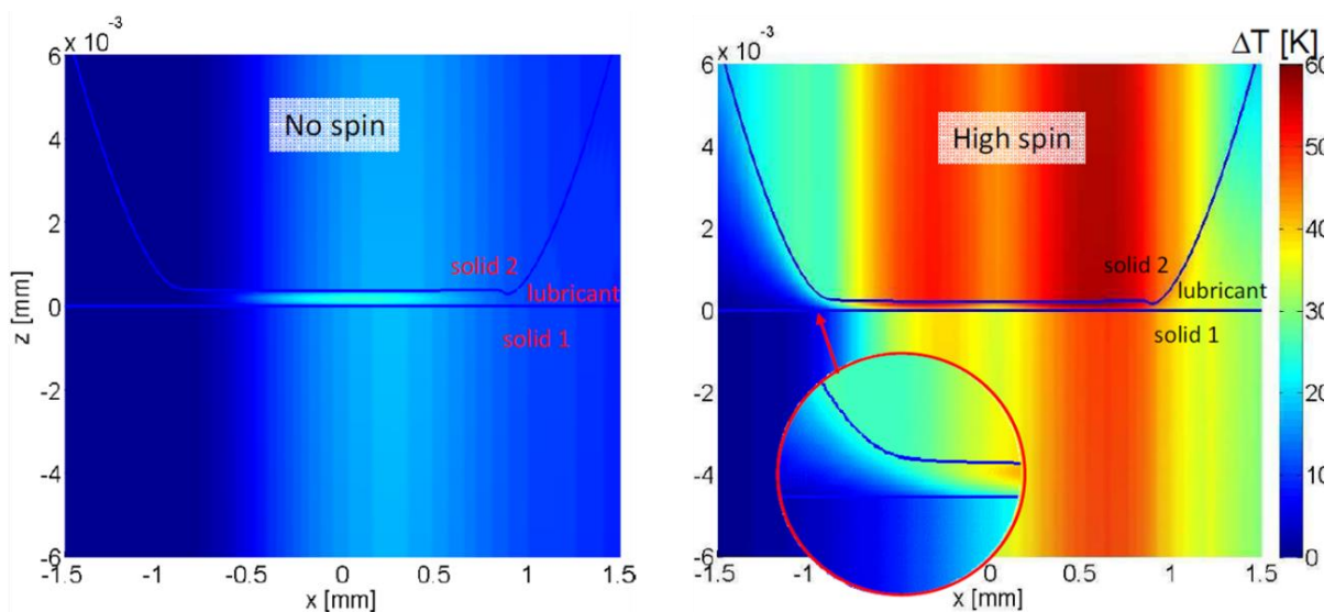
Figure 1.6. Temperature rise (colored area) and film thickness profiles (line) of the same contact with no spinning (left) and with spinning (right), from [7].
