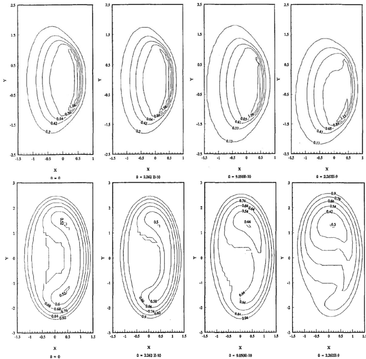
Figure 1.4. Contour plots of pressure (top) and film thickness (bottom) for different spin velocity values, from [13] (spinning increases from left to right).
