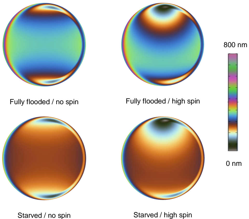
Figure 4.7. Numerical interferograms for four selected cases presented in Figure 7, for fully flooded and starved ( r_c = 1 ) conditions, without spinning and with high spinning ( B = 3.7 ).
