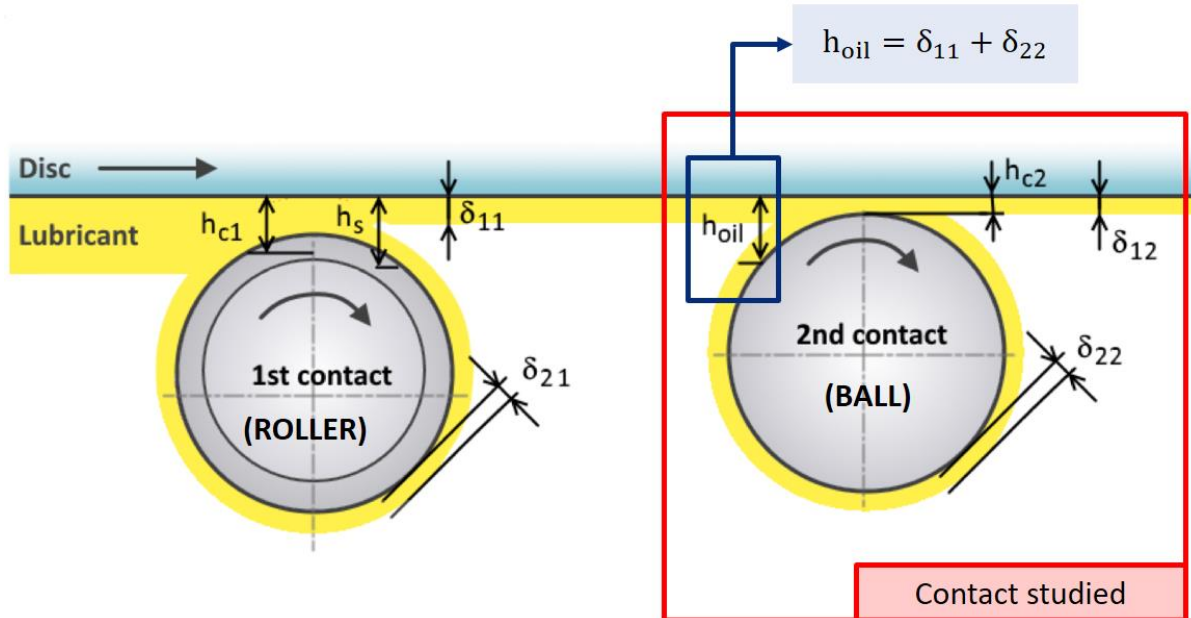
Figure 2.14. Schematic representation of the roller-ball-disk system (side view).
