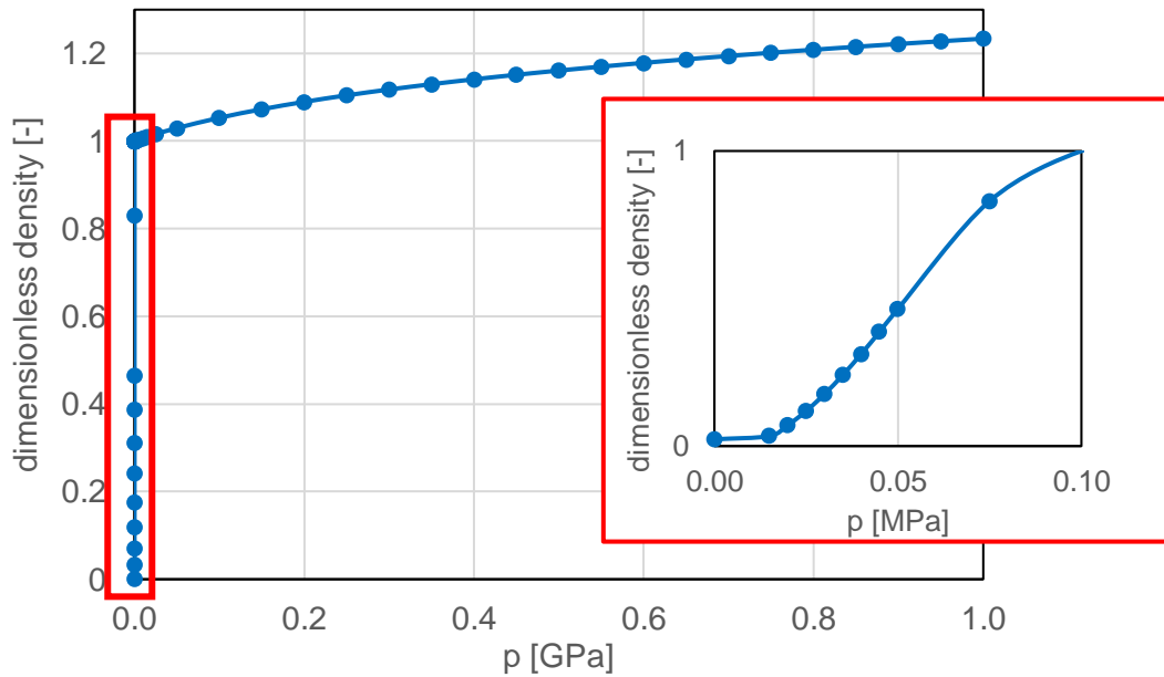
Figure 3.2. Dimensionless density \bar{\rho} ( \bar{\rho} = \rho/\rho_c ) variation with pressure of lubricant 2, following a similar representation as in [121]. The zoomed area indicates the low-to-high pressure transition.
