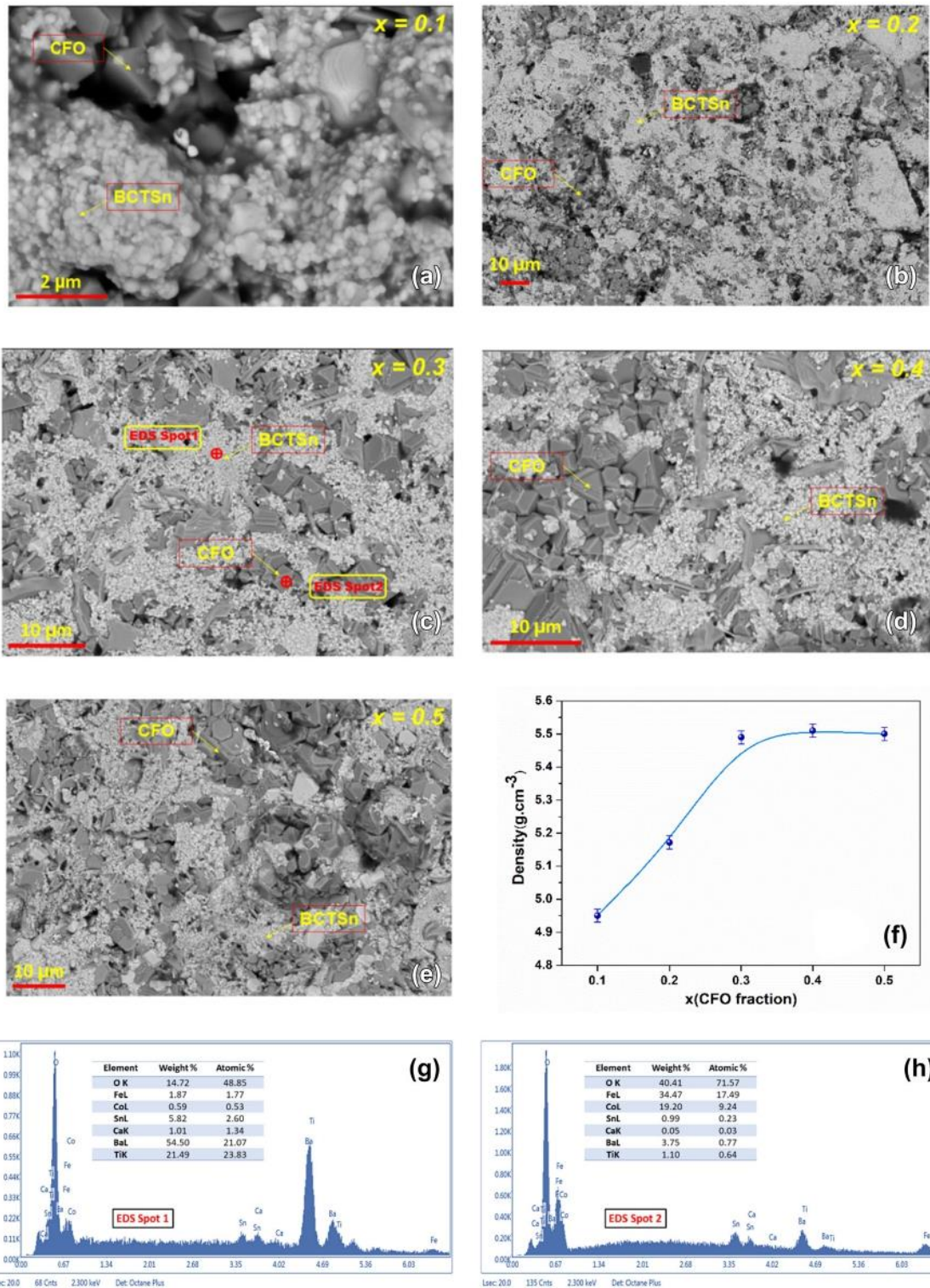
Fig. 5 a–e SEM micrographs, f bulk density as a function of ferrite content of various (1-x) BCTSn—(x) CFO composites and g and h EDS spectrum for composite with x = 0.3
