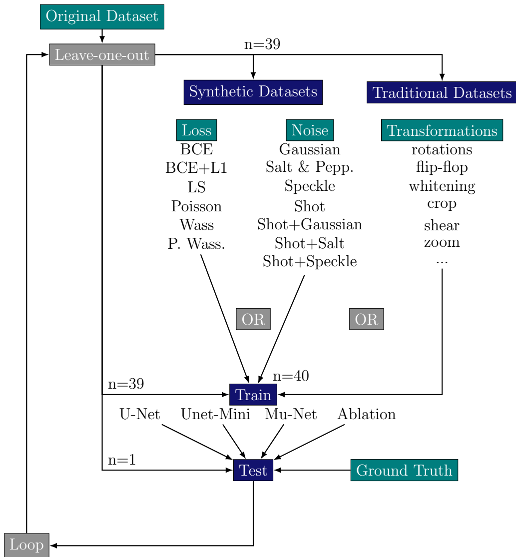
Figure 4.10: Experimental scheme of the leave-one-out strategy to test the effect of various data augmentation on segmentation. The synthetic and traditional datasets are generated at each loop without the leaved one out image.
