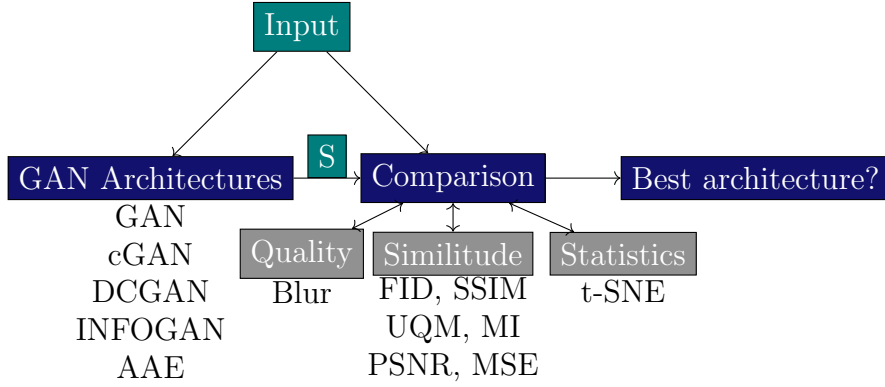
Figure 3.12: Procedure of GAN architecture comparison for the generation of bright-field brain organoid images. S corresponds to synthesised images.
