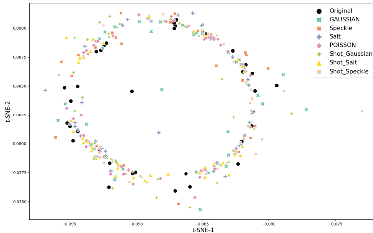
Figure 3.23: t-SNE representation of original and generated images with various noise injected in AAE.
