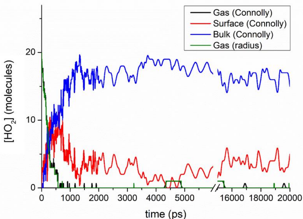
Figure 104: Time evolution of the HO 2 concentration in the gas phase determined by the radius method (green), and the gas phase (black), bulk (blue) and surface (red) concentrations determined by the Connolly method.
