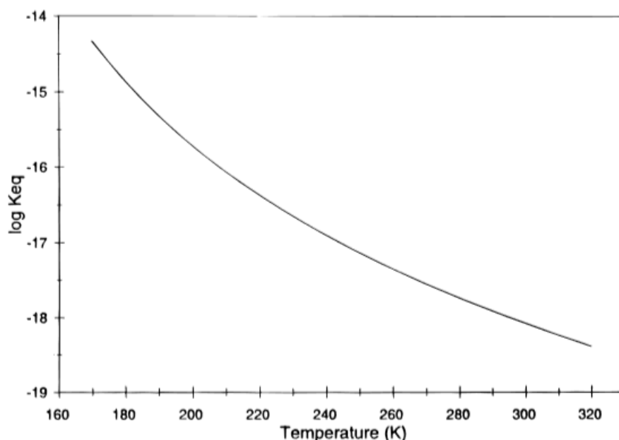
Figure 23: HO_2:H_2O equilibrium constant as a function of temperature. K_{eq} is in units of cm^3 molecule^{-1} taken from Aloisio and Francisco. 128
