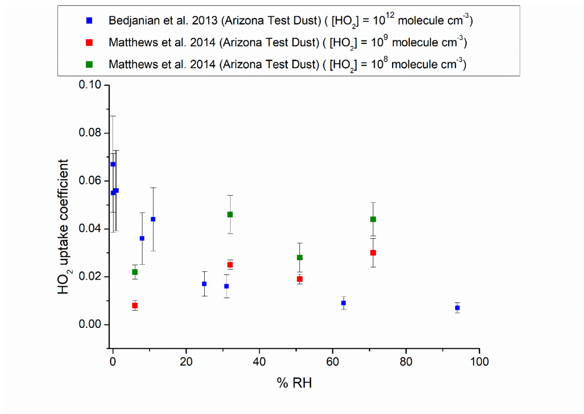
Figure 17: Influence of RH on the \text{HO}_2 uptake for Arizona Test Dust. 56,61
