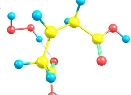
Figure 118: Geometries of the reactive Van der Waals complexes (RC) and product Van der Waals complex (PC) of the four different hydrogen environments.
