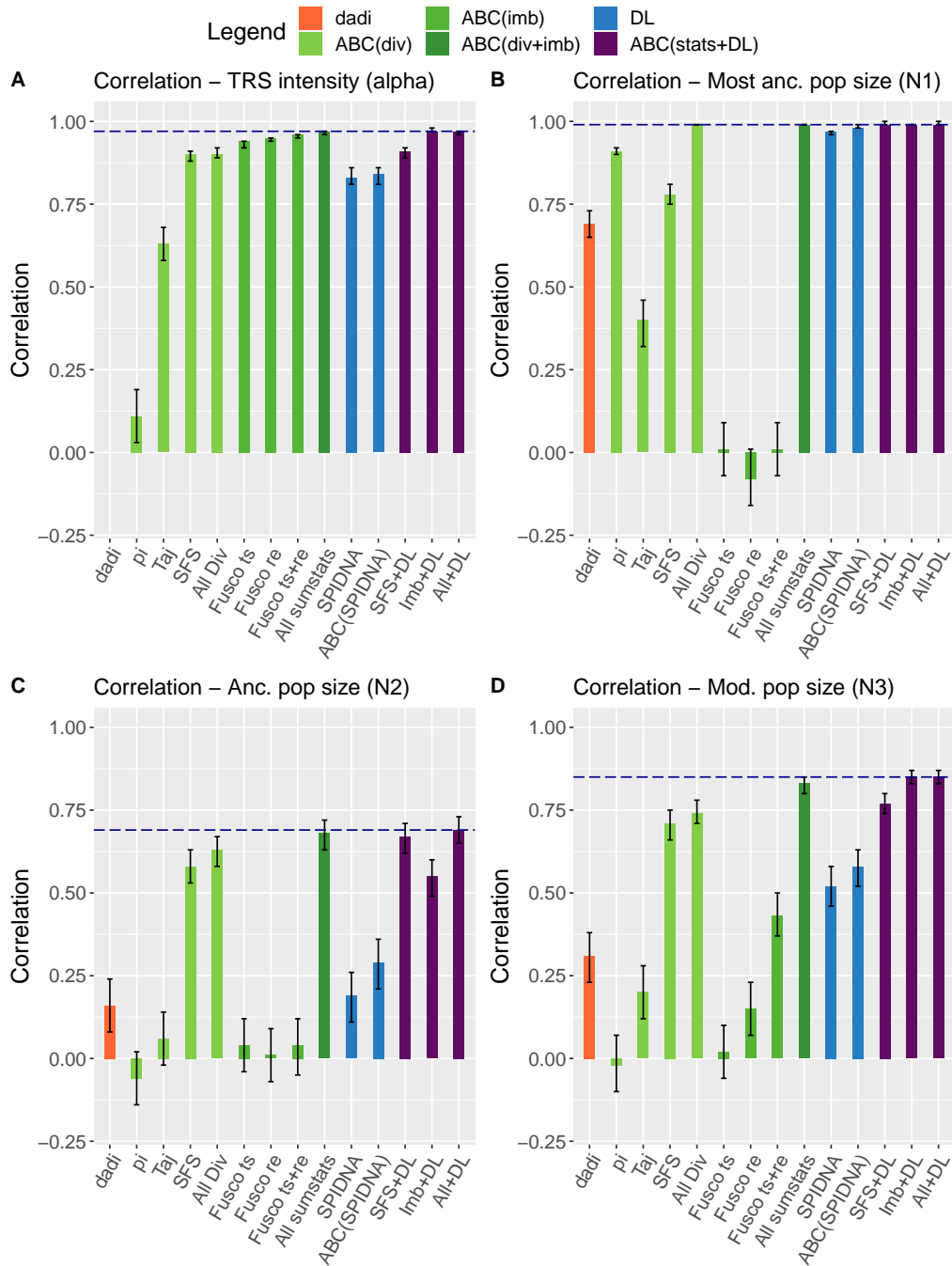
Figure 3.2: Comparison of inference methods accuracy using correlations.
