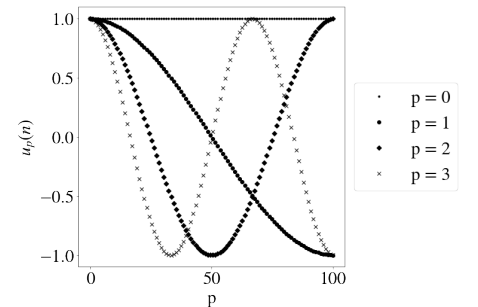
Figure 1.4: The first 4 basis functions u_p(n) .
