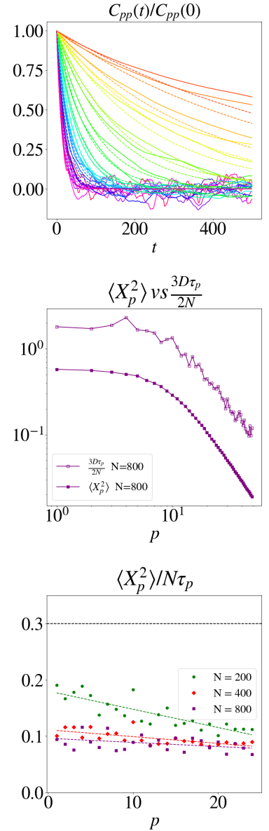
Figure 6.4: Top panel: the correlation function of mode p \in [1 \dots 25] function of time, C_{pp}(t) for a globule of length N = 200 .
