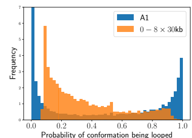
Figure 4.18: Histogram of the probability of a single measurement configuration being looped, for loop region A1 and for the non-looped region 0 - 8 \times 30\text{kb} .
