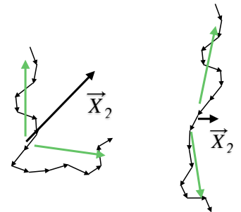
Figure 1.6: Illustrative examples of \tilde{\vec{X}}_2 , which is the sum of the two green vectors.
