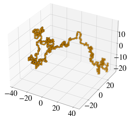
Figure 3.3: A single conformation of a coil
