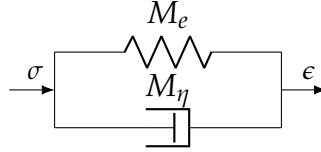
Figure II.5: Illustration of the Kelvin-Voigt viscoelastic rheologic model.
