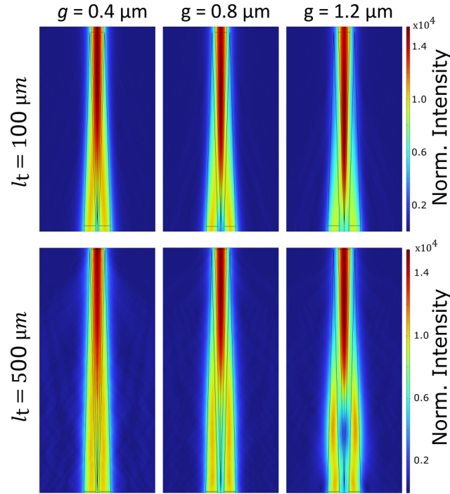
Figure 3.4: Adiabatic criterion simulations for 1 to 2 splitters. Simulations with l_t = 100 \mu m (top panel) and l_t = 500 \mu m (bottom panel) and gap distances g \in \{0.4, 0.8, 1.2\} \mu m (left to right panels). As in the experiments, full optical splitting is achieved for larger l_t . Simulations done in 2D via COMSOL Multiphysics considering \Delta n \approx 5 \times 10^{-3} .
