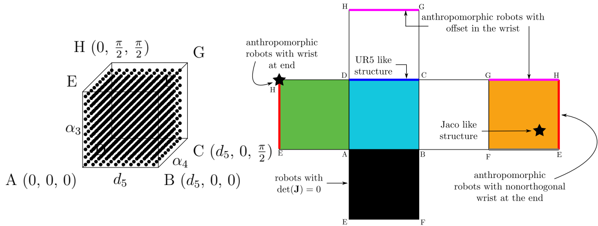
Figure 3.17 – Classification of a 6R robot parameterized in specially chosen three D-H parameters. The rest of the DH parameters match that of FANUC CRX-10ia/L robot.
