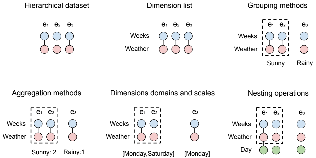
Figure 4.3: Data abstraction in GRIDIFY. Dimension list consists of two implicit relations (Weeks and Weather). Grouping the geo-coded entities ( e.g. , e_1 , e_2 , and e_3 ) based on the Weather dimension achieves two groups. One group contains e_1 and e_2 that only has Sunny value. In contrast, another group contains e_3 that only has Rainy value. Aggregation method estimates the statistic of grouped groups ( e.g. , one group has two elements and another has one element). Dimension domain method shows the value scales from other dimensions ( e.g. , one group has a domain in [Monday, Saturday] ). Nesting operations generate another level nest ( e.g. , adding the Day dimension).
