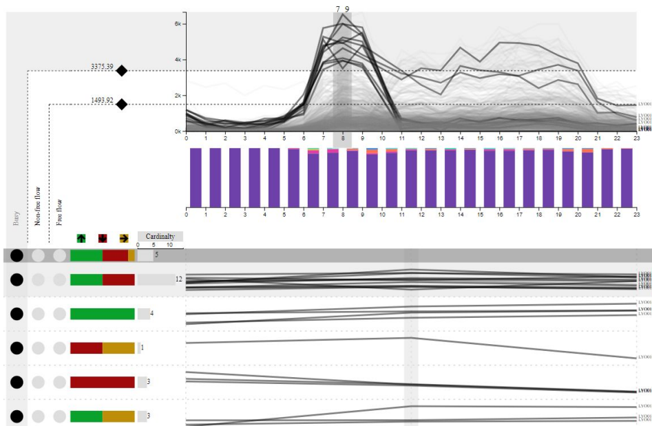
Figure 5.8: The traffic flow patterns during morning peak. An aggregated group with 5 subgroups reaches the peak time in the morning, but some do not reach the peak in the evening.
