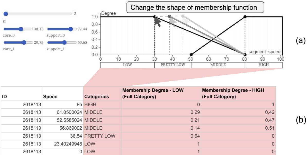
Figure 3.4: The illustration of interaction on FuzzyCut. Users can adjust the shape of the membership function by dragging the black points on the membership function as illustrated with three arrows or dragging the parameter sliders (blue) shown on the left in (a). Based on the membership function shapes, it can create categories with different labels (LOW, PRETTY LOW, MIDDLE, HIGH). The data format and the derived new attributes are in table (b). The raw data includes the quantitative data speed and derived attributes, including Categories and the membership degrees , such as the columns Membership Degree - LOW (Full Category) and Membership Degree - HIGH (Full Category) .
