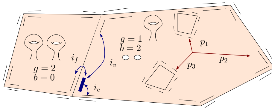
FIGURE 5.4: An example of extended combinatorial map, with the three involutions i_v , i_e , and i_f for a given flag (in bold), and the pointers p_1 , p_2 and p_3 between a face and one flag for each incident cycle
